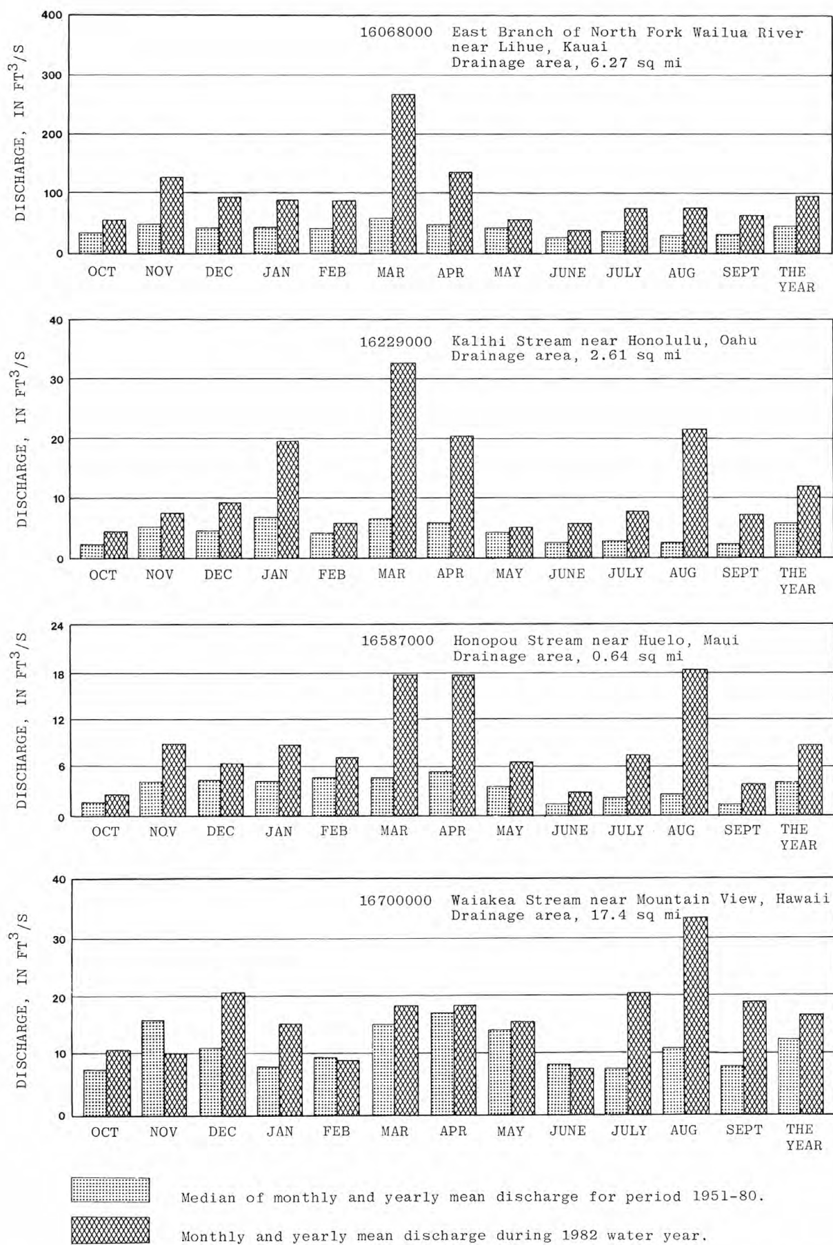
FIGURE 1. DISCHARGE DURING 1982 WATER YEAR COMPARED WITH MEDIAN DISCHARGE FOR PERIOD 1951-80 FOR FOUR REPRESENTATIVE GAGING STATIONS.
