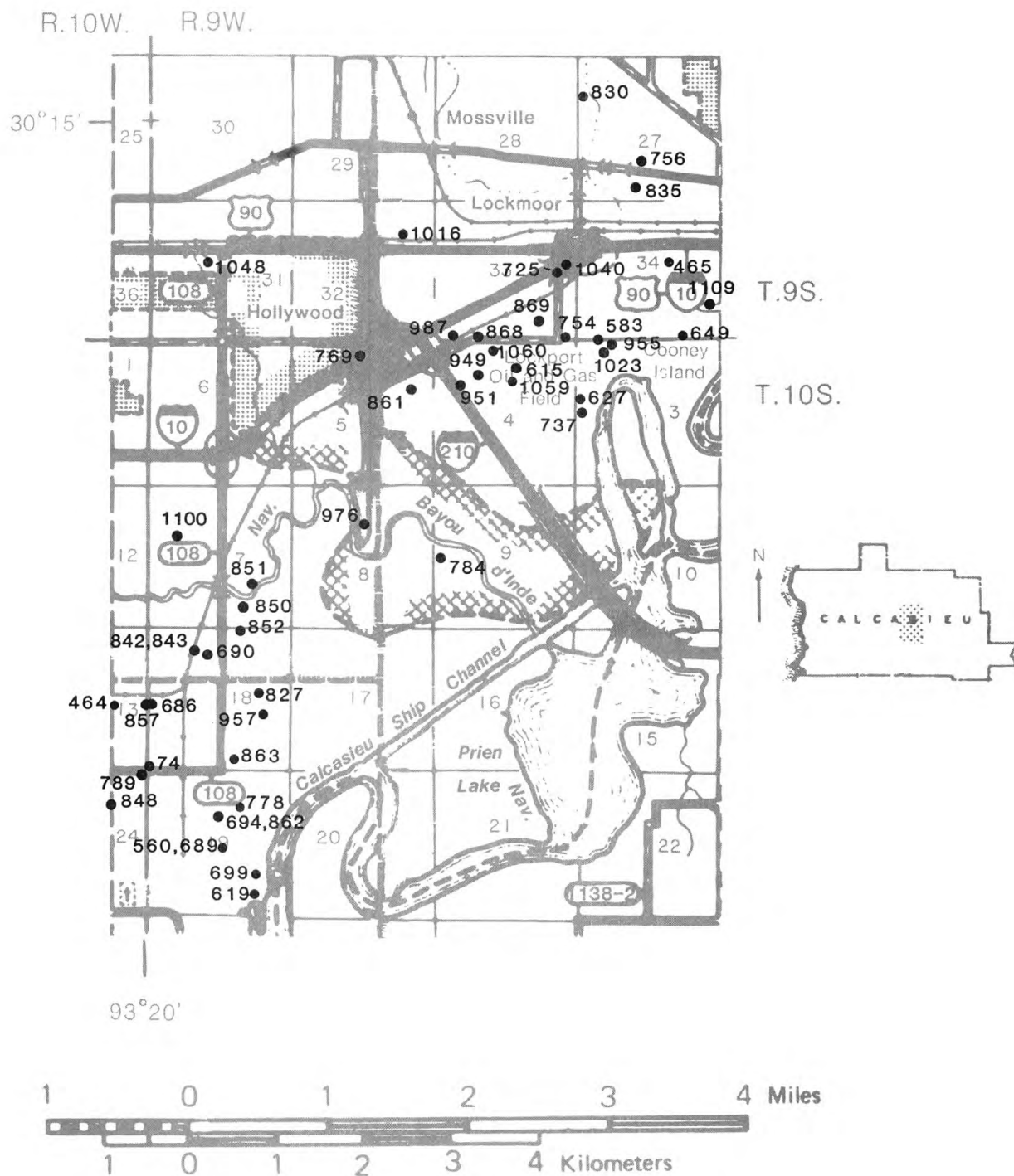
Figure 16.--Location of wells for which water-quality data are included in the shaded area shown in figure 15, Calcasieu Parish.
