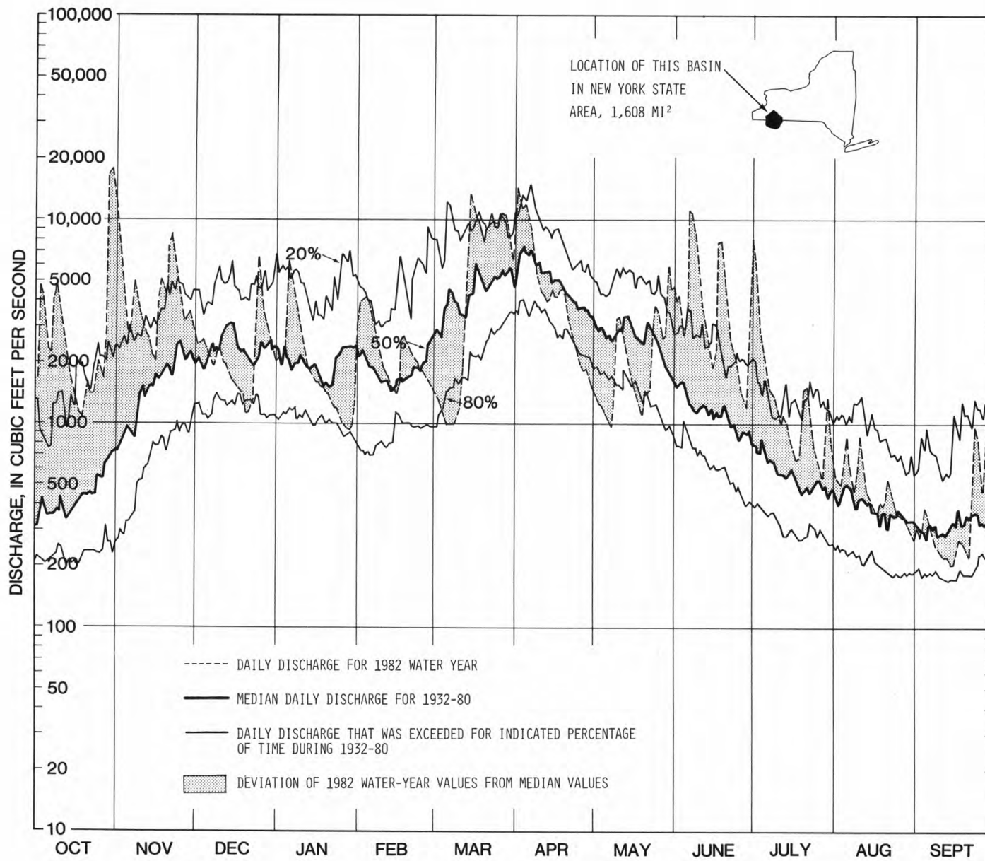
Figure 3.--Hydrographic comparisons, Allegheny River at Salamanca, N.Y.
