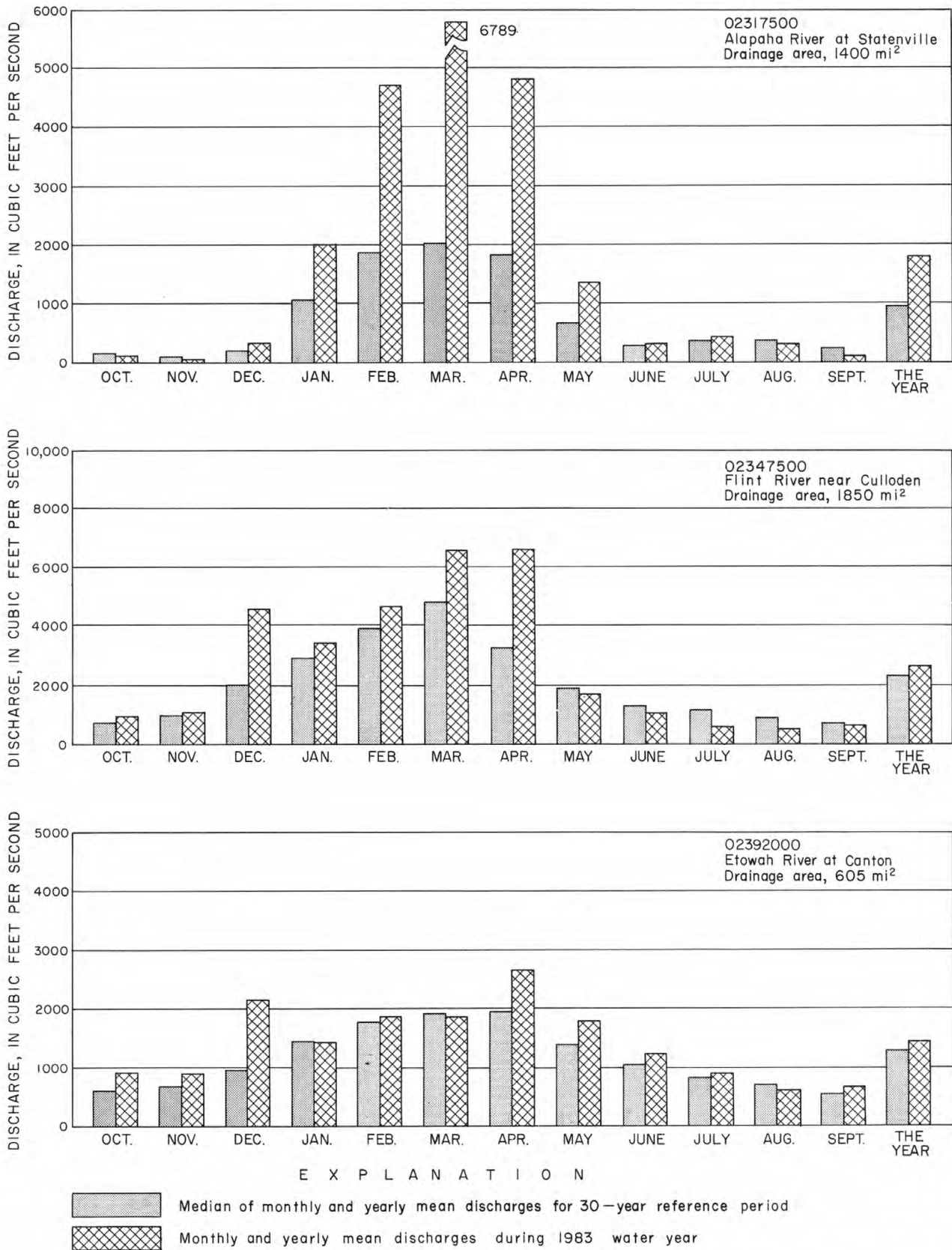
Figure 1.—Comparison of discharge at three representative long-term gaging stations during 1983 water year with median discharge for 30-year reference period.
