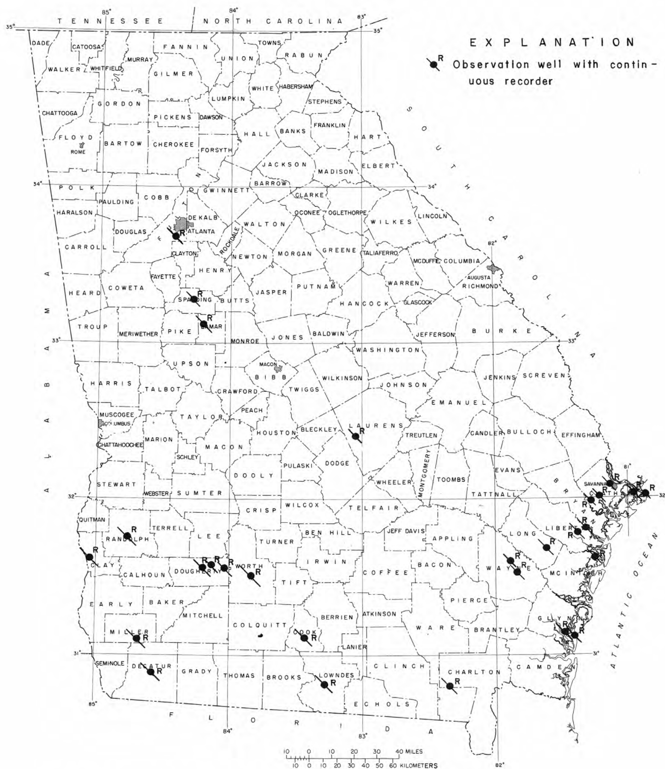
Figure 7.—Location of selected observation wells.
