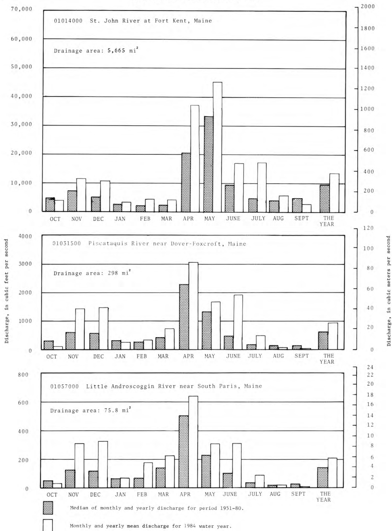
Figure 2.-- Comparison of discharge at three long-term index gaging stations during 1984 water year with median discharge for period 1951-80.
