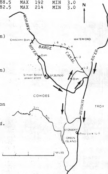
Figure 5.--Gaging stations and diversions near mouth of Mohawk River.
