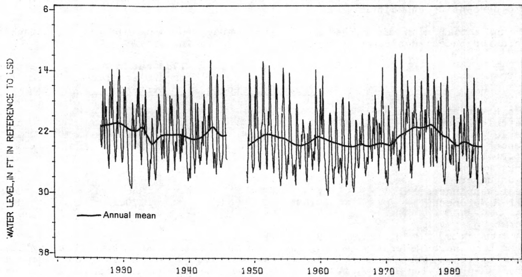
HYDROGRAPH B.--Well Oe-151, Oneida County, period of record
