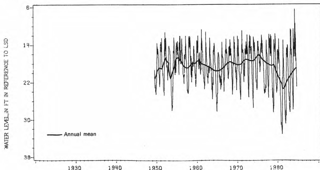
HYDROGRAPH A.--Well Ro-18, Rockland County, period of record
