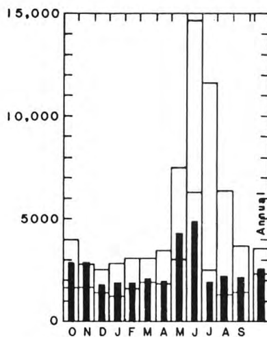
06279500 Bighorn River at Kane, 1930-83
