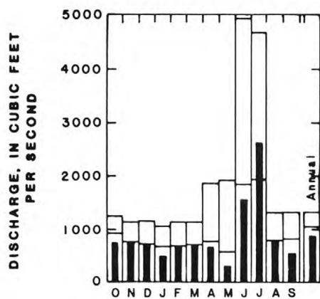
06285100 Shoshone River near Lovell, 1967-83
