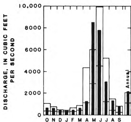
06630000 North Platte River above Seminole Reservoir, near Sinclair, 1939-83
