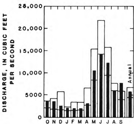
13022500 Snake River above Reservoir near Alpine, 1954-83
