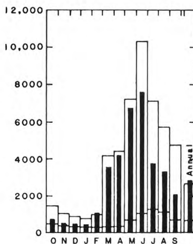
06674500 North Platte River at Wyoming-Nebraska State line, 1929-83
