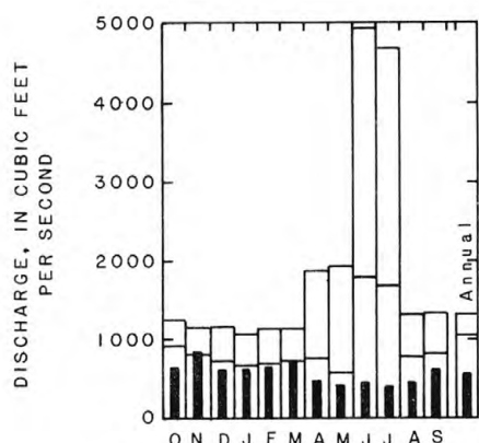
06285100 Shoshone River near Lovell, 1967-84
