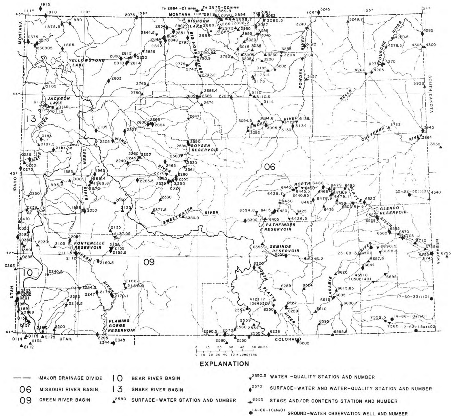
Figure 1.—Map showing locations of lake- and stream-gaging stations, water-quality stations, and ground-water observation wells, 1985 water year.
