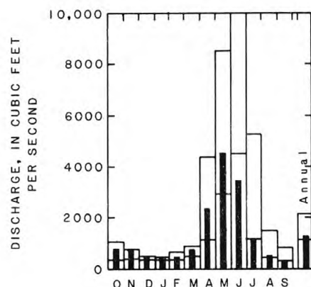
06630000 North Platte River above Seminoe Reservoir, near Sinclair, 1939-84
