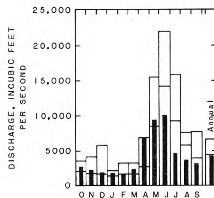
13022500 Snake River above Reservoir near Alpine, 1954-84
