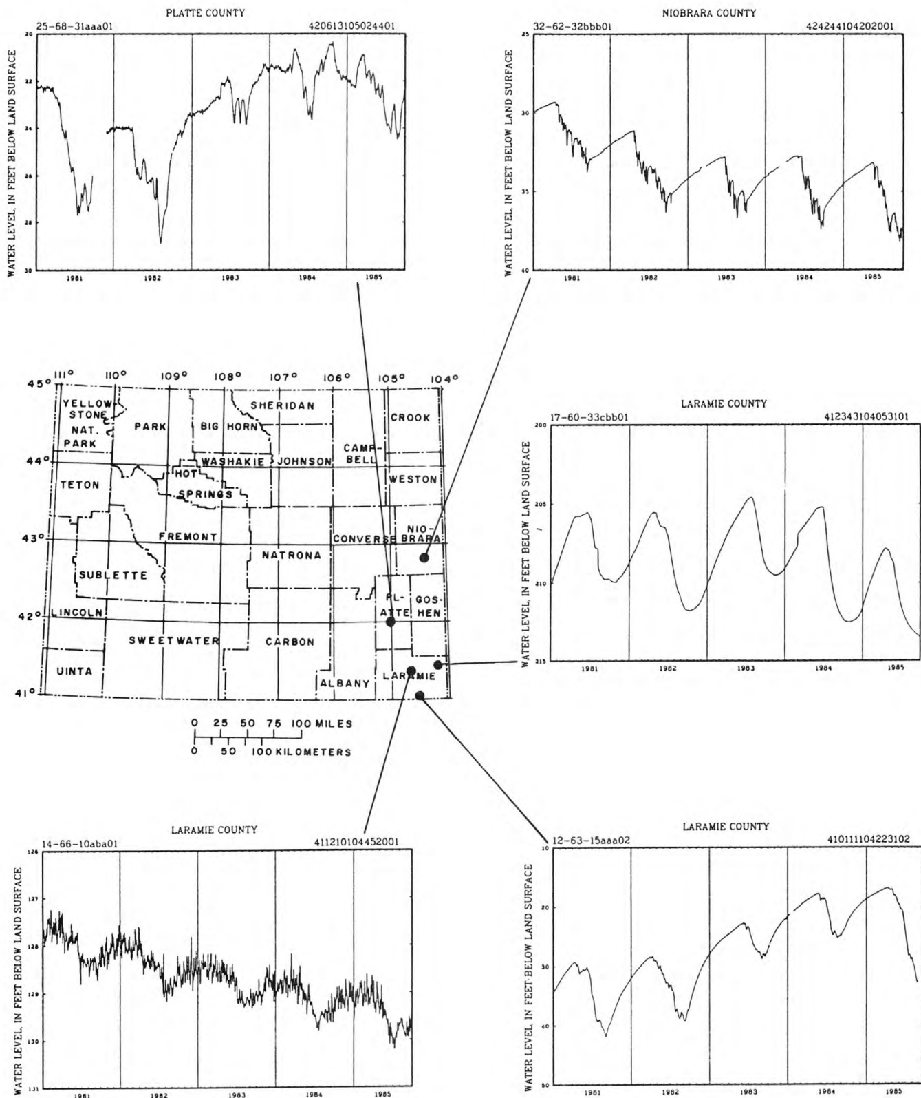
Figure 4.--Water-level fluctuations from January 1981 to September 1985 in observation wells located in areas of extensive ground-water withdrawals.
