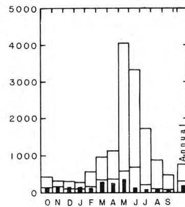
06317000 Powder River at Arvada, 1931-84
