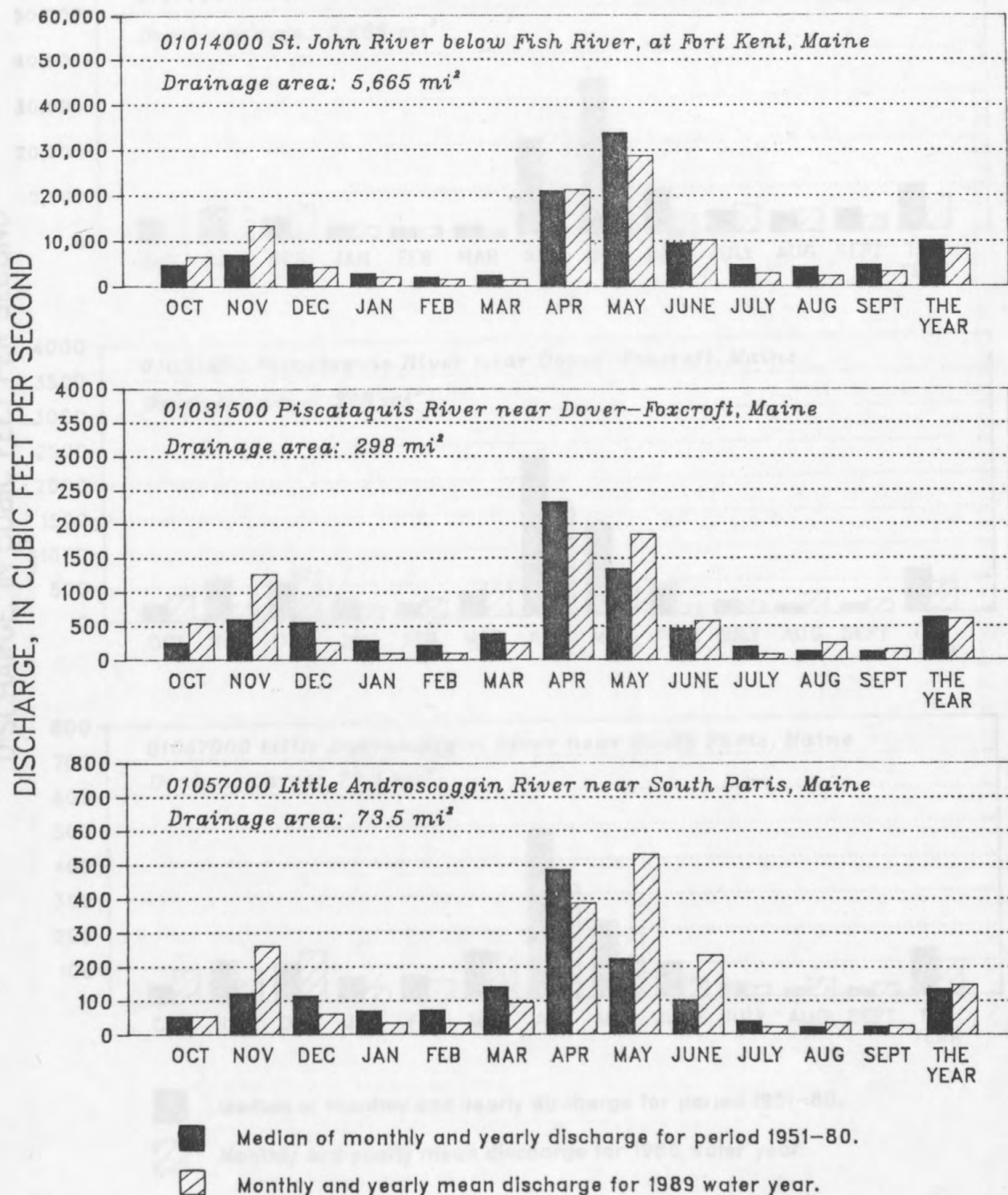
Figure 3.—Comparison of discharge at three long-term index gaging stations during 1989 water year with median discharge for period 1951-80.
