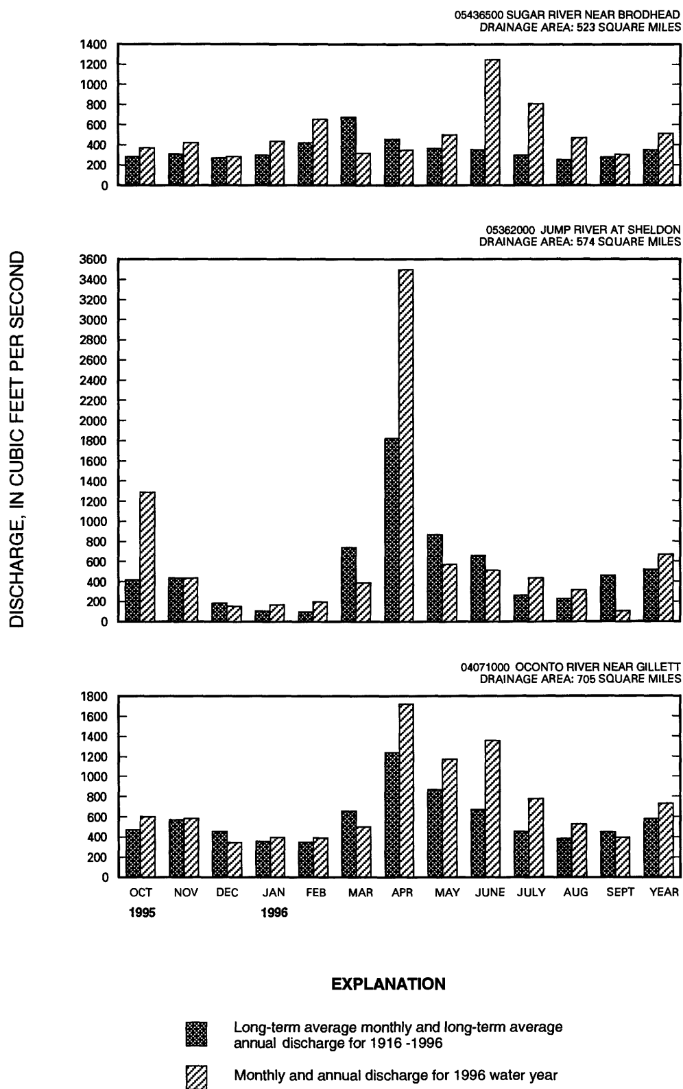
Figure 3. Comparison of discharge at representative gaging stations during 1996 water year with discharge for 1916 -1996.
