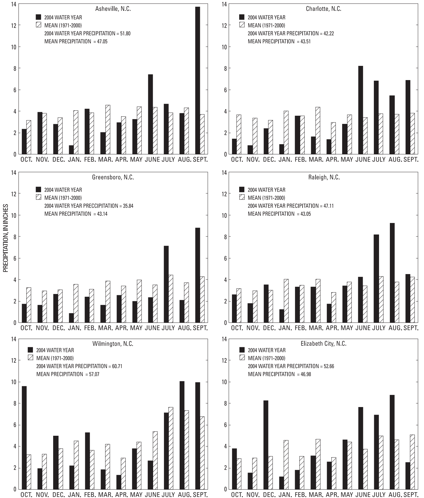
Figure 3.--Monthly precipitation for the 2004 water year and mean monthly precipitation for the period 1971-2000 at index stations across North Carolina (data from the National Oceanic and Atmospheric Administration).
