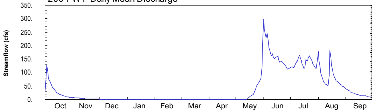
2004 WY Daily Mean Discharge
