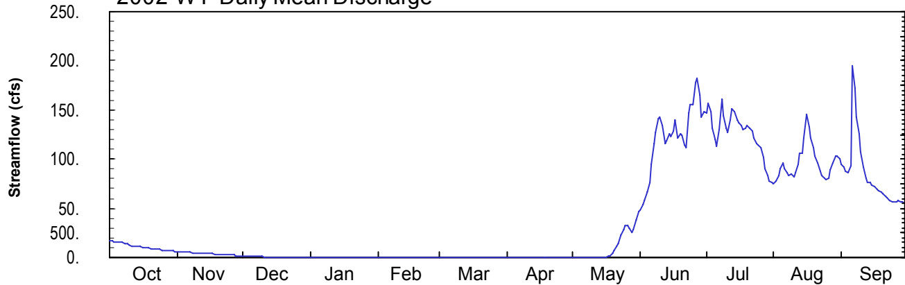
2003 WY Daily Mean Discharge
