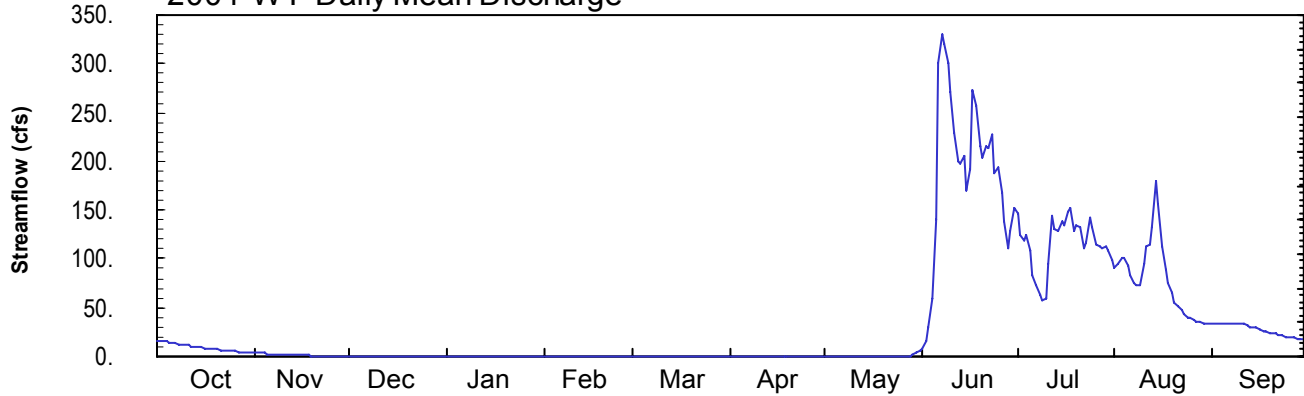
2002 WY Daily Mean Discharge
