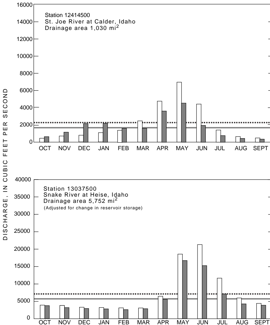
Figure 1. Discharge during 2005 water year compared with median discharge for period 1971-2000 for four representative gaging stations.
