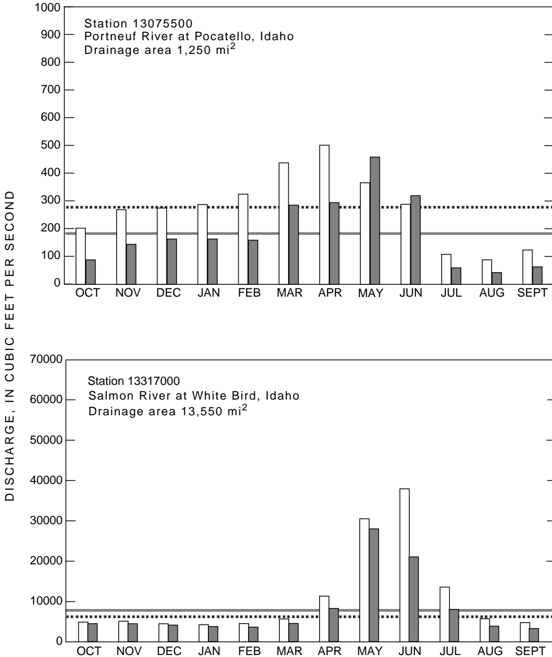
Figure 1. Discharge during 2005 water year compared with median discharge for period 1971-2000 for four representative gaging stations--Continued.
