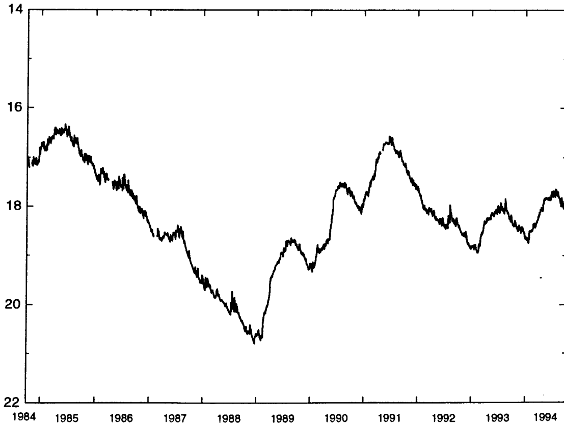
Figure 3.--Water level at observation well 381034085502601
