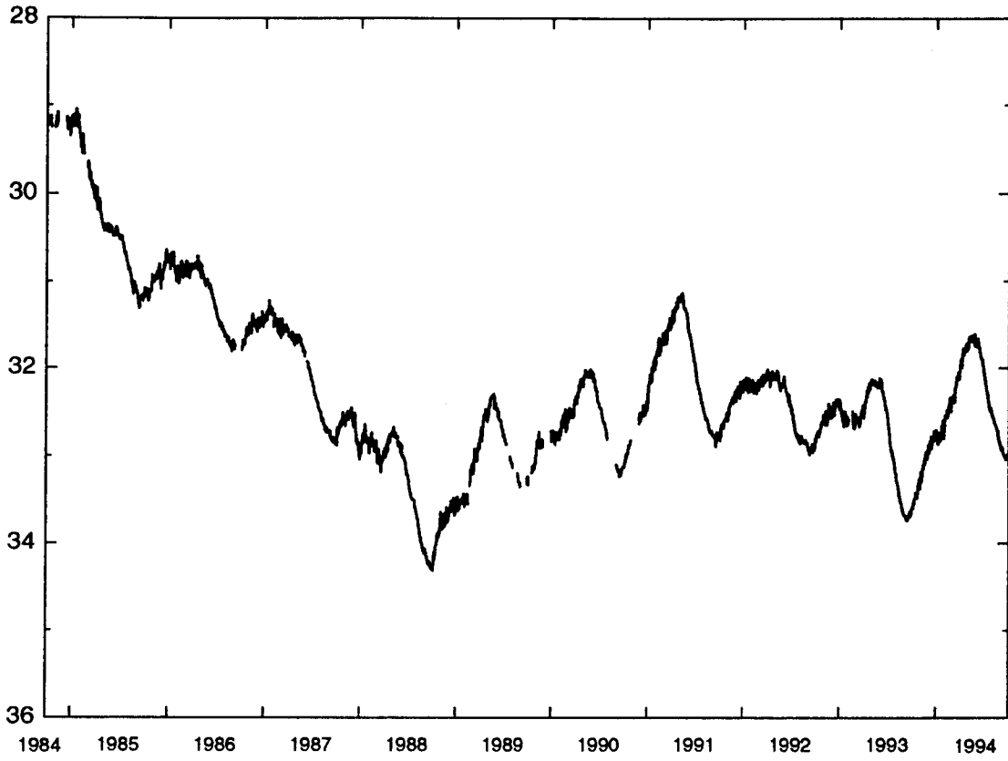
Figure 2.--Water level at observation well 381447085454001
