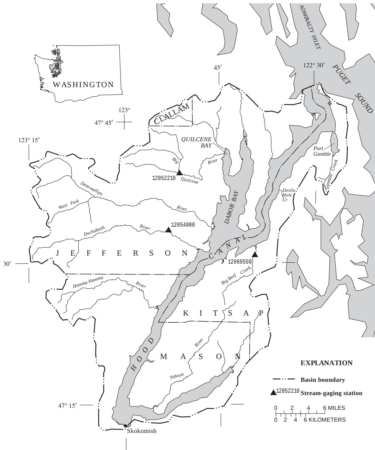
Figure 13. Location of surface-water stations in the Big Quilcene River, Duckabush River, and Big Beef Creek Basins.
