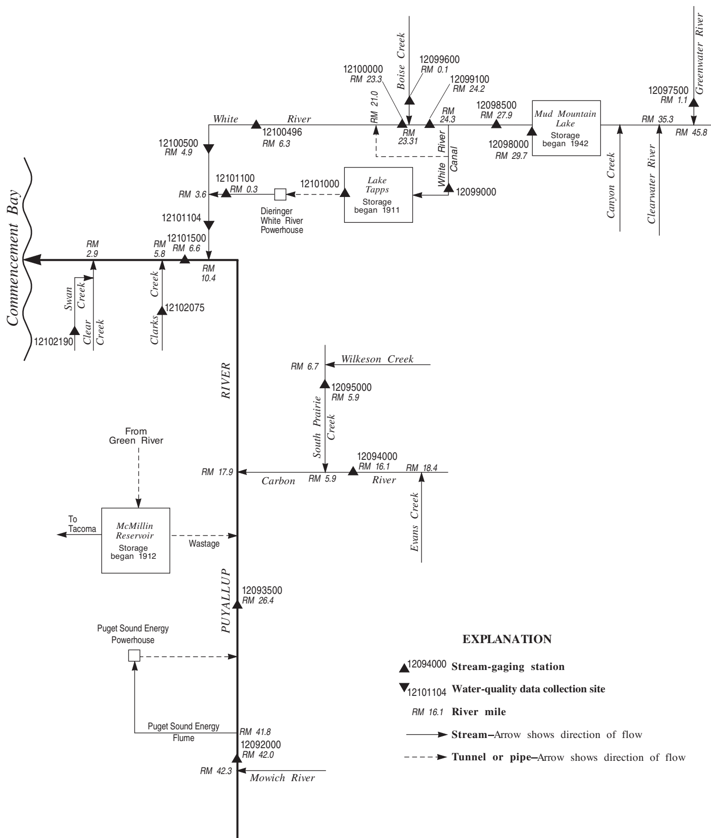
Figure 24. Schematic diagram showing surface-water and water-quality stations in the Puyallup River Basin.
