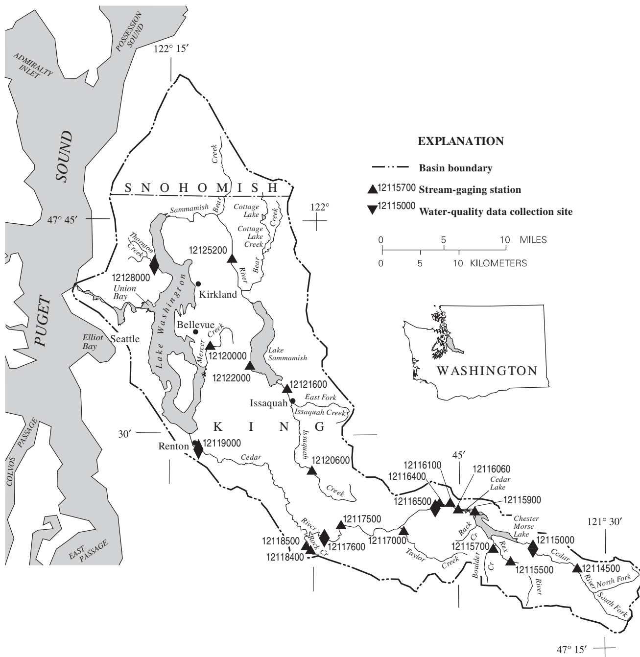
Figure 27. Location of surface-water and water-quality stations in the Lake Washington and Sammamish River Basins.
