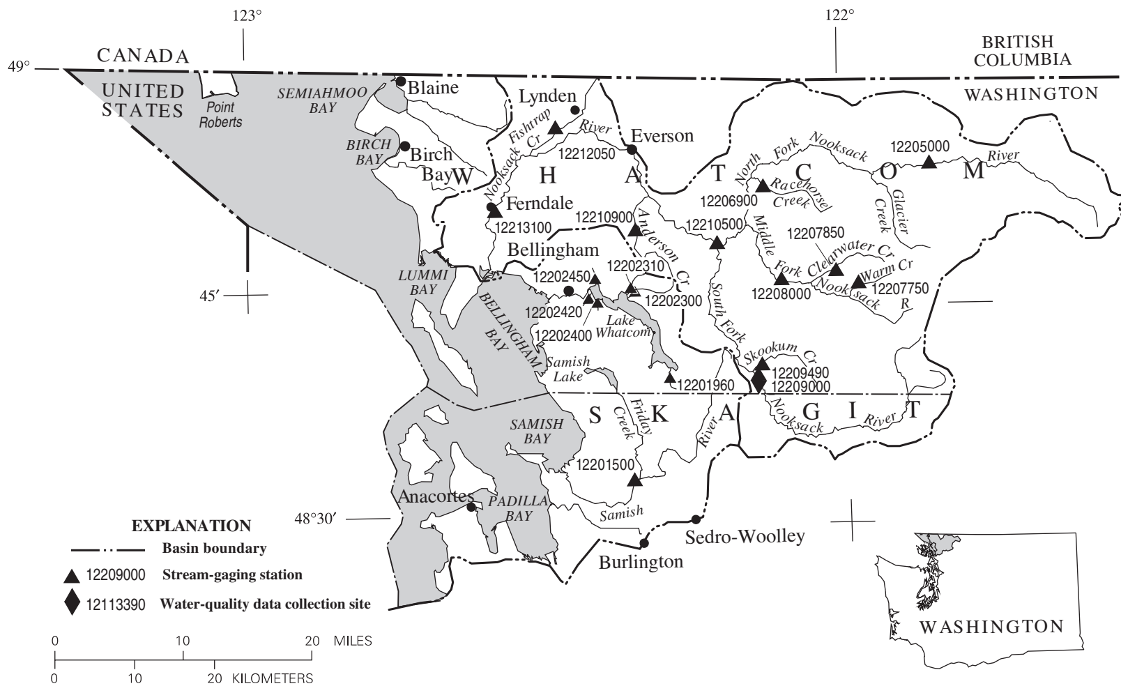
Figure 33. Location of surface-water stations in the Nooksack River and Samish River Basins.
