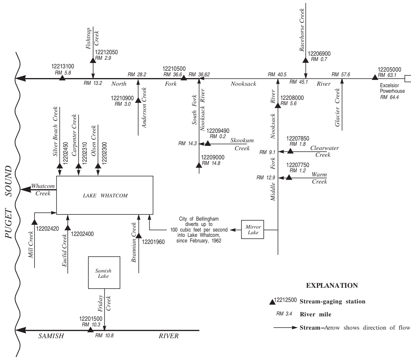
Figure 34. Schematic diagram showing surface-water stations in the Nooksack River and Samish River Basins.
