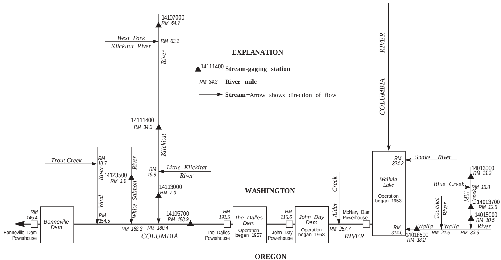
Figure 48. Schematic diagram showing surface-water stations in the Columbia River Basin between Wallula Lake and Stevenson including Walla Walla, Klickitat, and White Salmon River Basins.
