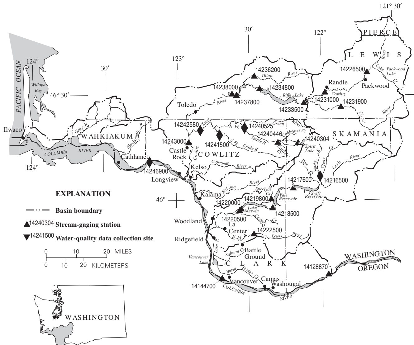
Figure 49. Location of surface-water and water-quality stations in the Lewis and Cowlitz River Basins and downstream to mouth of Columbia River.
