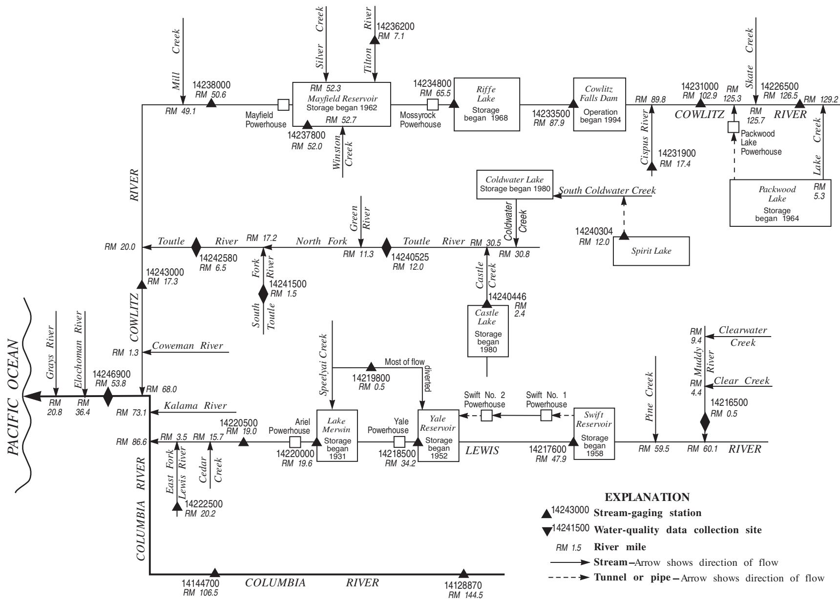
Figure 50. Schematic diagram showing surface-water and water-quality stations in the Lewis and Cowlitz River Basins and downstream to mouth of Columbia River.
