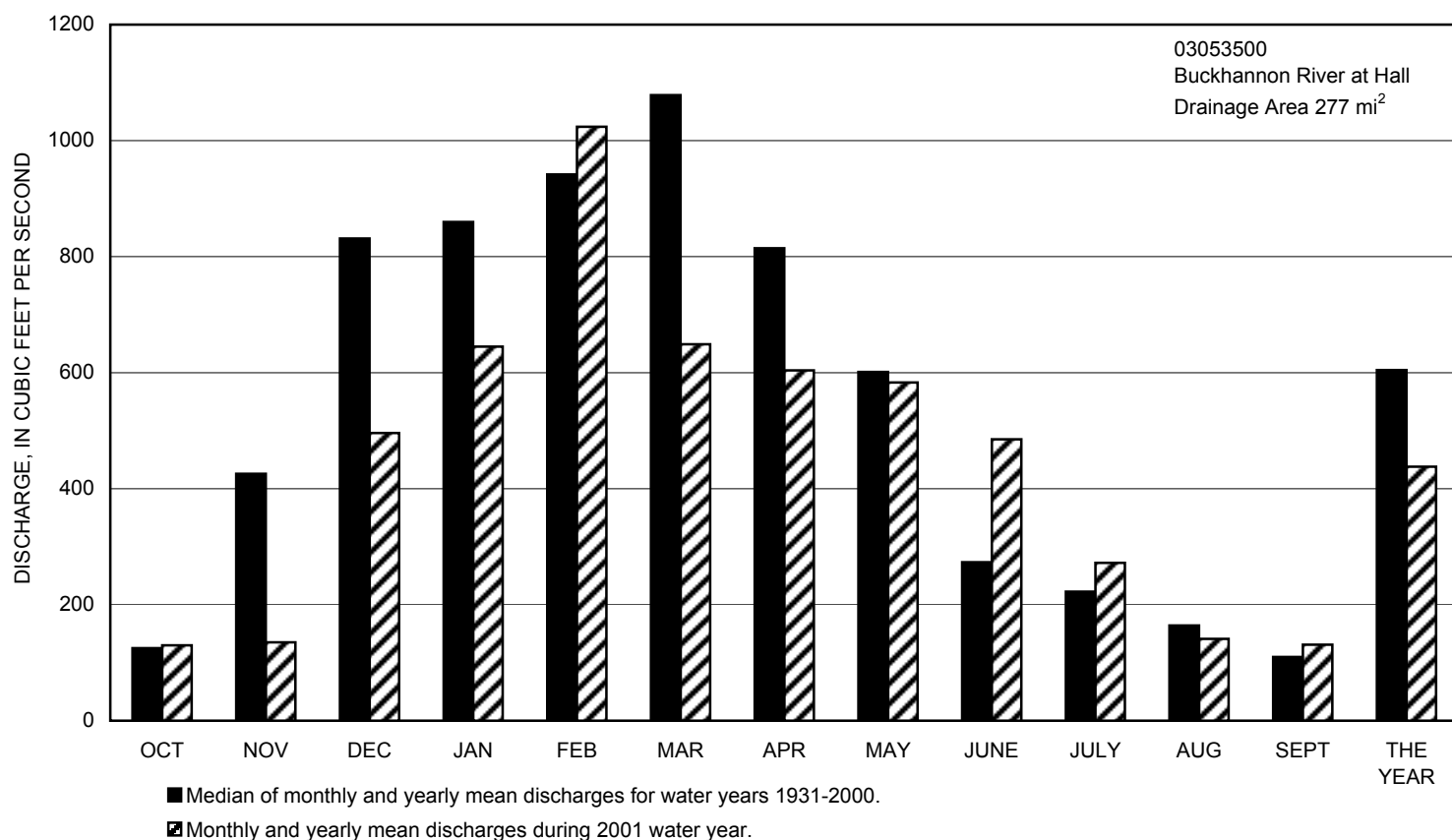
Figure 1.--Discharge at the South Branch Potomac River and the Buckhannon River index gaging stations during the 2001 water year compared to median discharge for the period 1931-2000.
