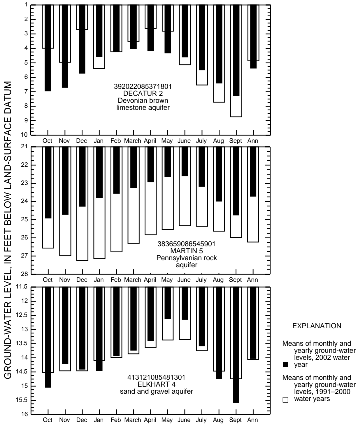
Figure 4. --Monthly and yearly mean of daily minimum ground-water levels at three Indiana ground-water-observation wells during water-year 2002 and mean of monthly and yearly minimum ground-water levels for period of 1991-2000.
