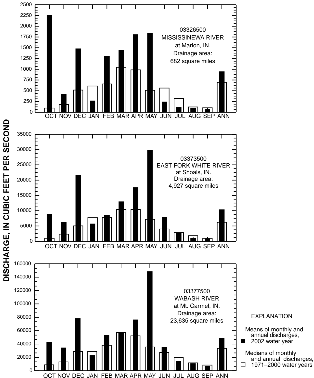
Figure 3. --Mean discharge at three Indiana streamflow-gaging stations during water-year 2002 and median discharges for period of 1971-2000.
