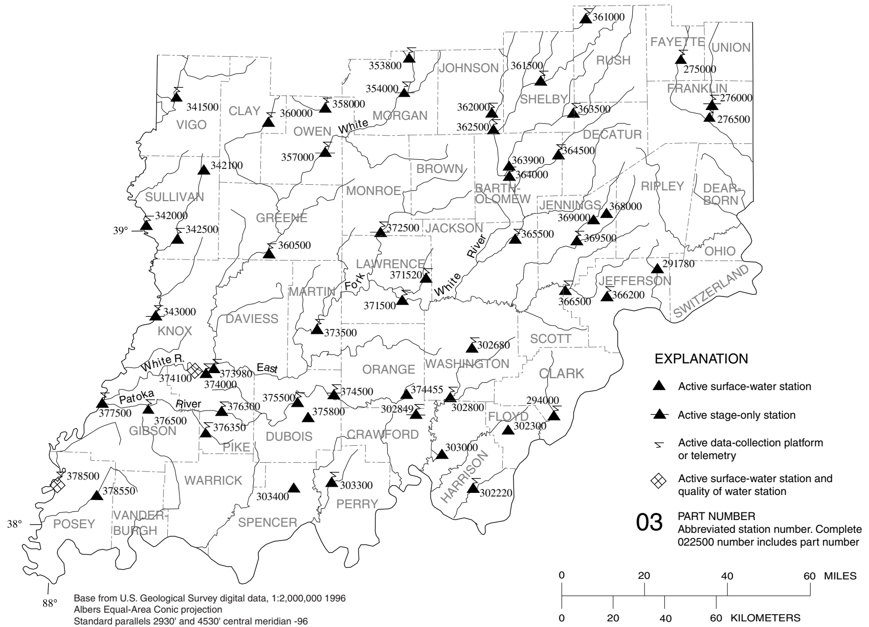
Figure 6.--Locations of streamflow and water-quality gaging stations in Indiana.
