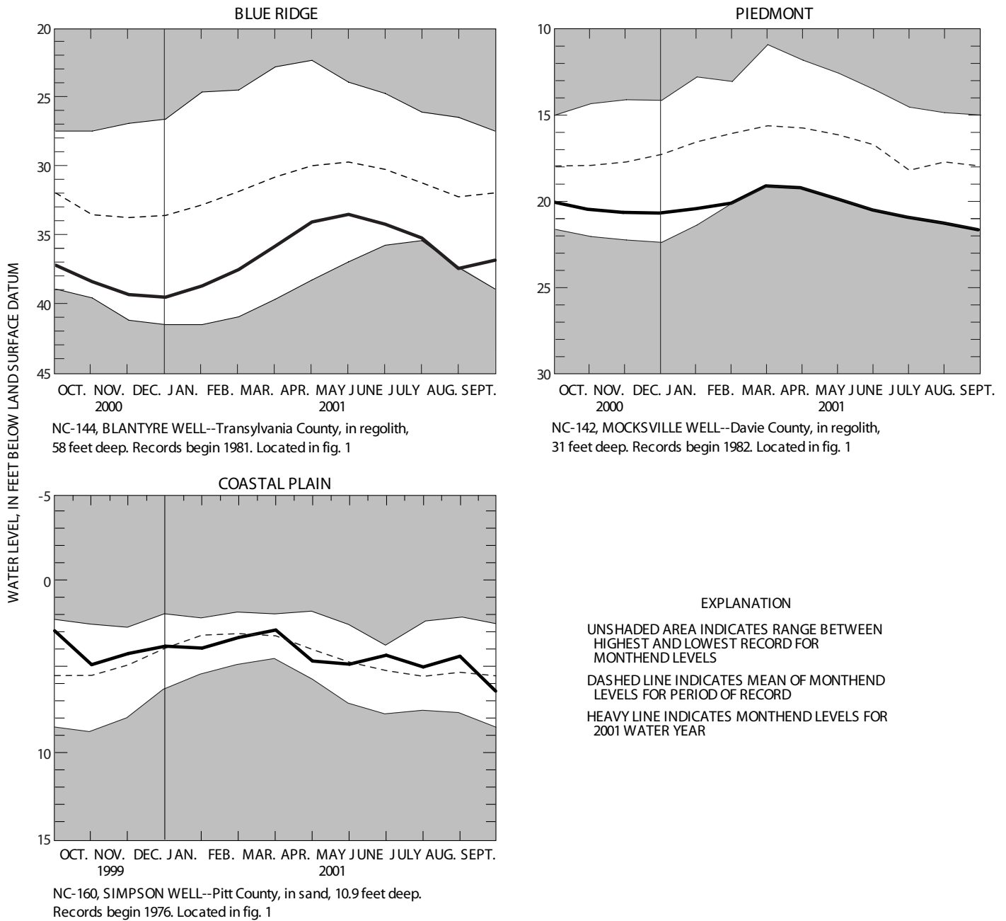
Figure 11.--Water levels in index observation wells in the Blue Ridge, Piedmont, and Coastal Plain Provinces.
