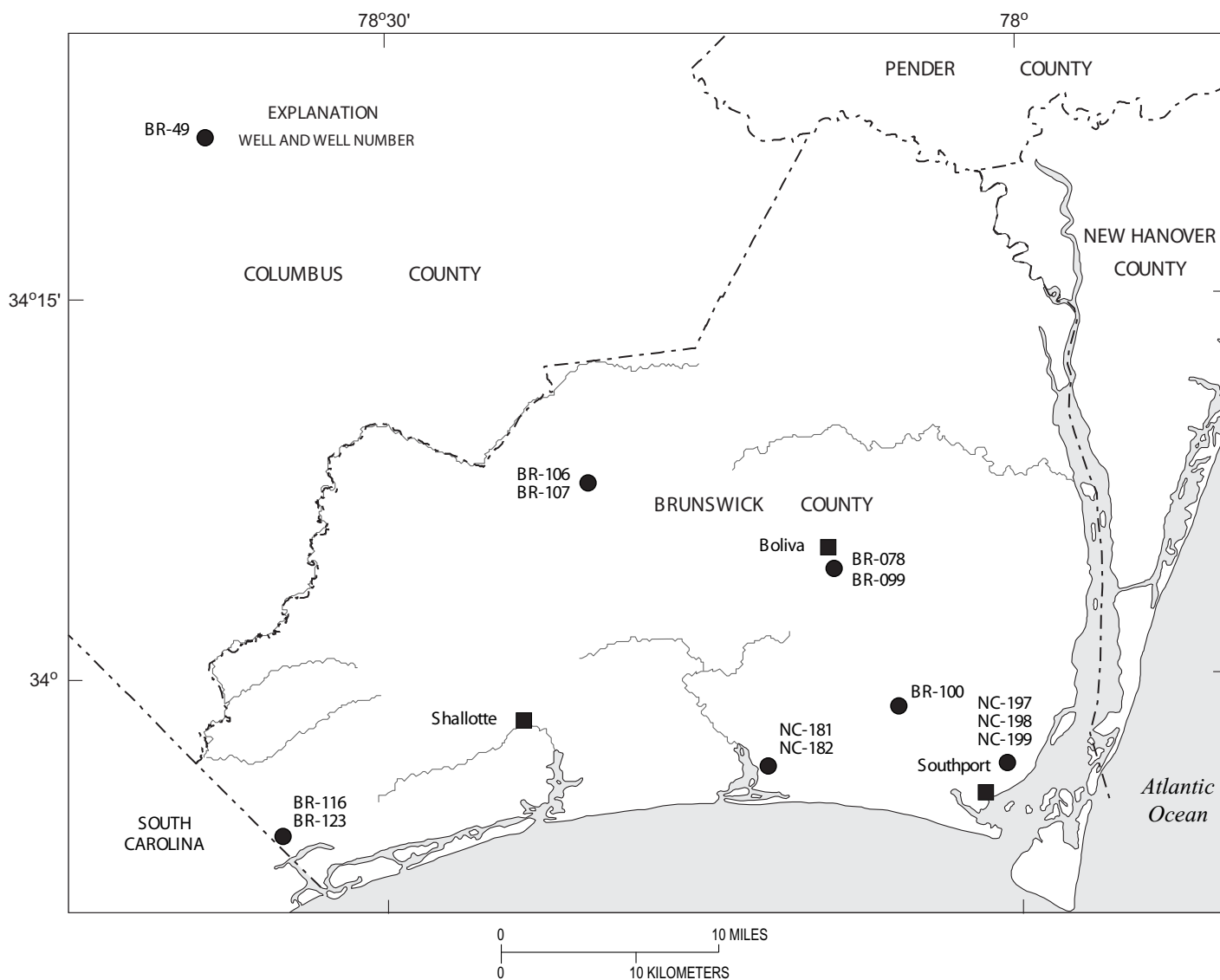
Figure 4.--Location of observation wells in Brunswick County.
