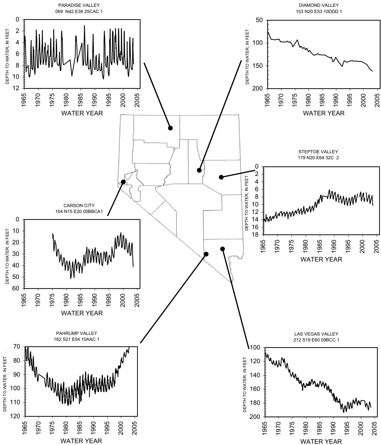
Figure 7. Long-term water-level depths below land surface in six selected observation wells.
