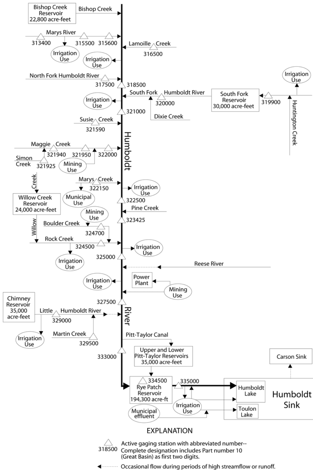
Figure 25. Schematic diagram of flow system and gaging stations in the Humboldt River basin.
