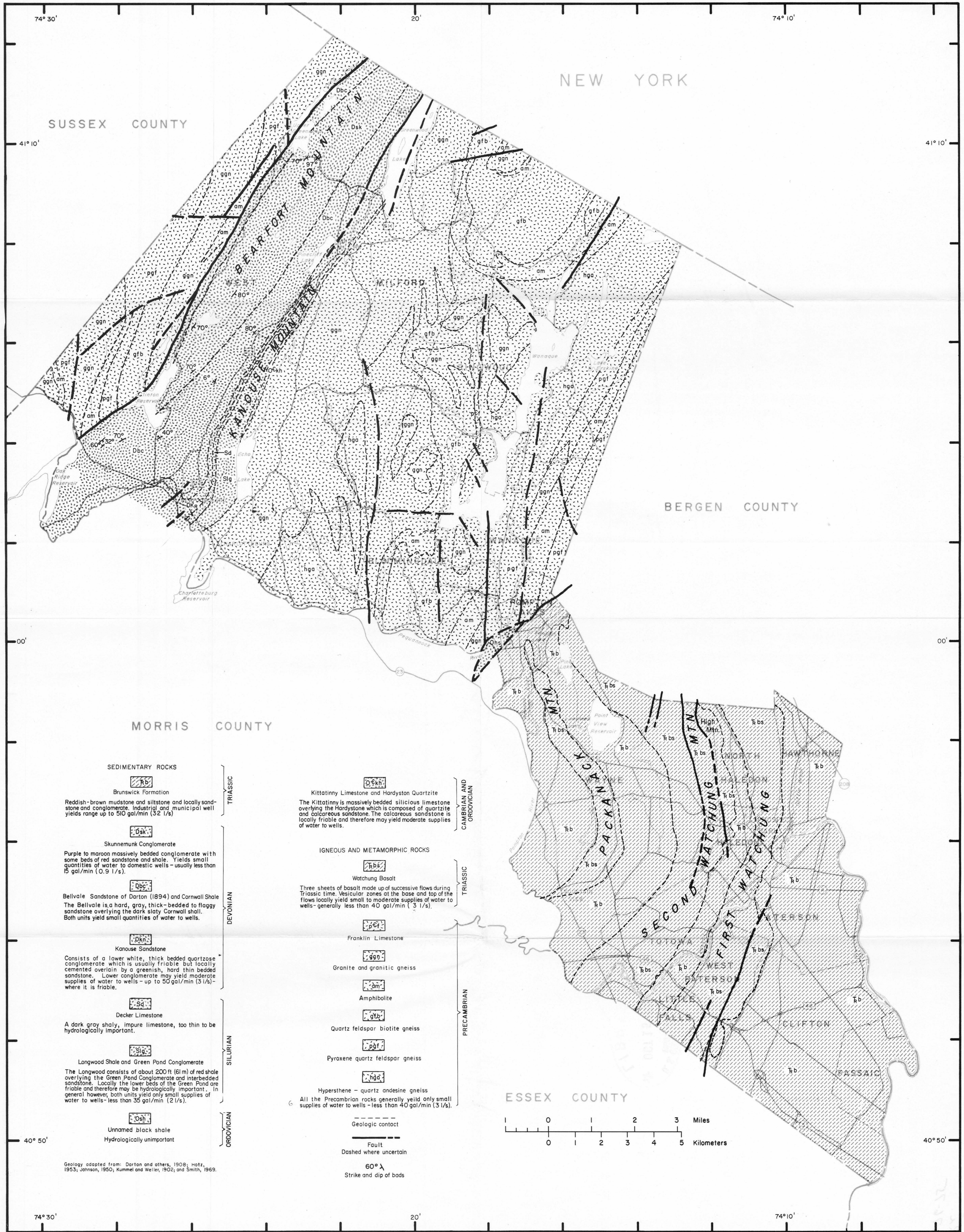
Figure 3 -- Geologic map of Passaic County, New Jersey
