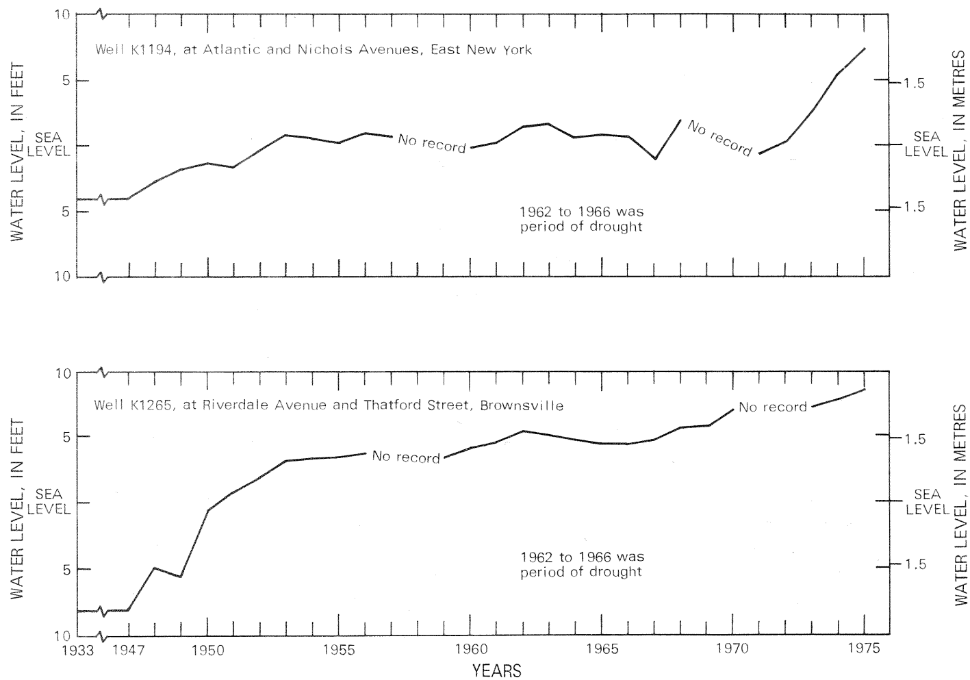
Figure 8.--Average water-table altitudes at observation wells in East New York and Brownsville, Kings County, N.Y., from 1933 to 1976.
