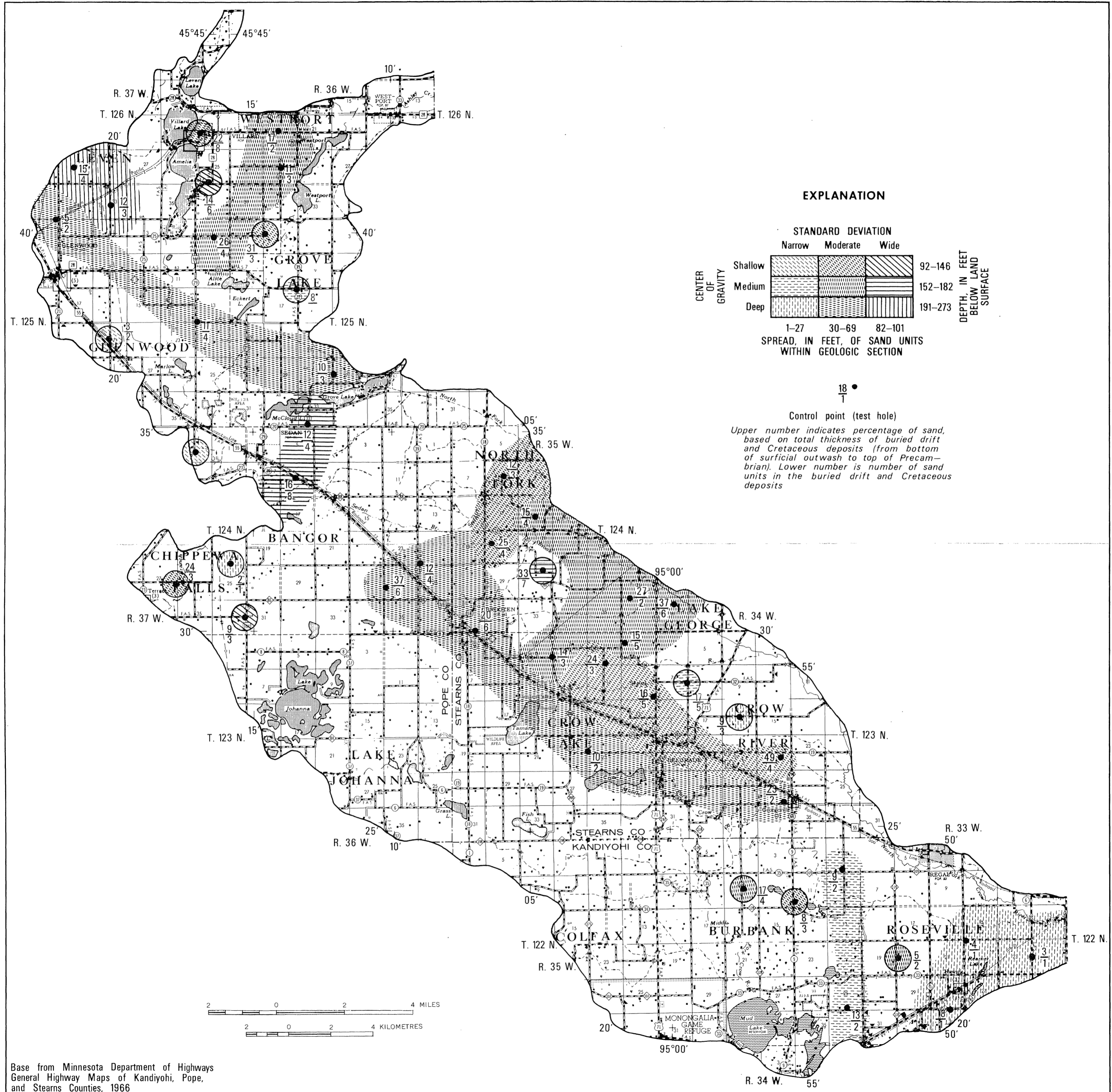
Plate 6.--Distribution of sand units 4 or more feet thick in the buried drift and Cretaceous deposits.
