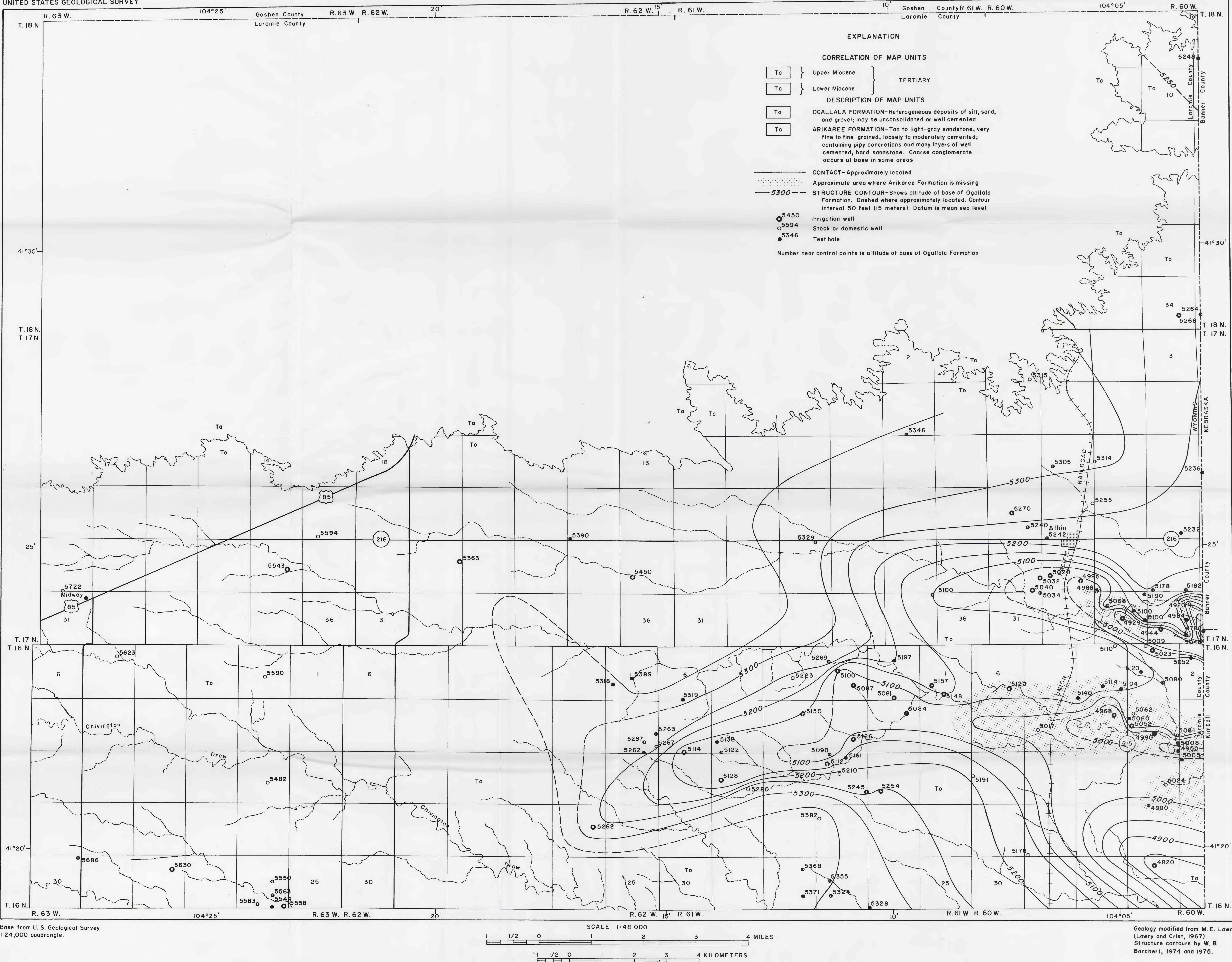
FIGURE 3.—MAP SHOWING GEOLOGY AND STRUCTURE CONTOURS ON BASE OF OGALLALA FORMATION IN THE ALBIN AREA, SOUTHEASTERN WYOMING
