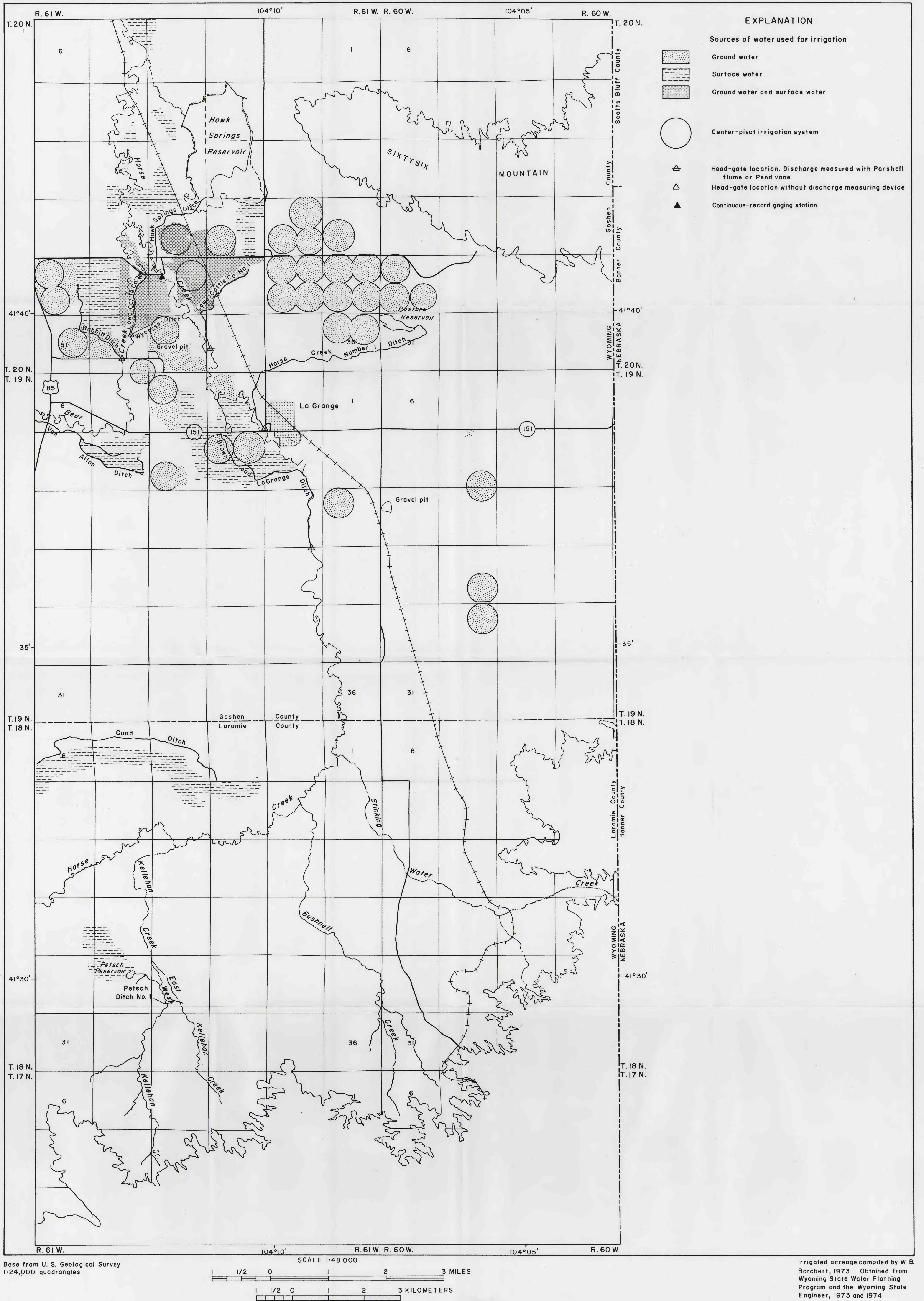
FIGURE 14.--IRRIGATED ACREAGE IN THE LA GRANGE AREA, SOUTHEASTERN WYOMING, 1974
