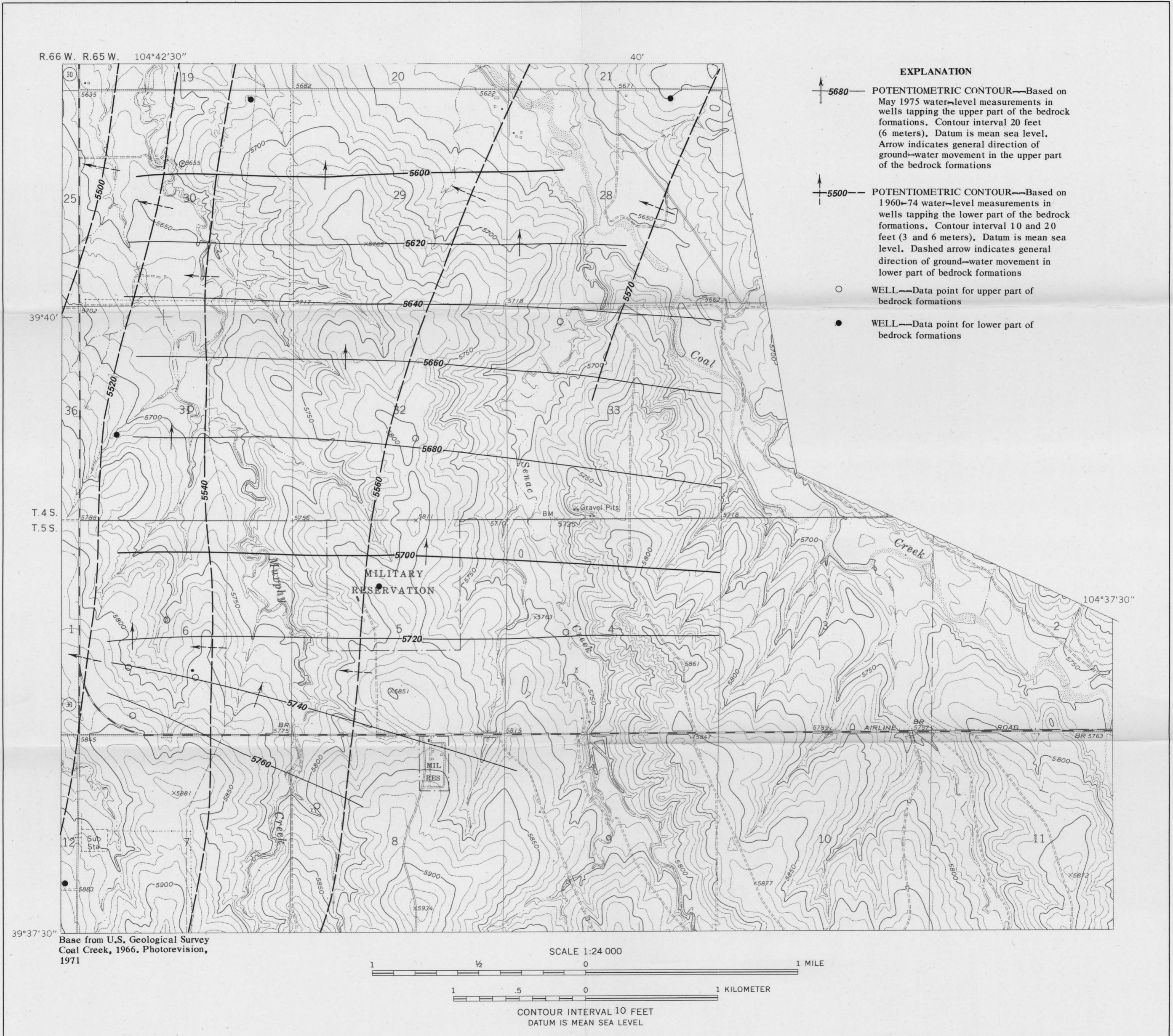
MAP SHOWING POTENTIOMETRIC CONTOURS FOR THE UPPER AND LOWER PARTS OF THE BEDROCK FORMATIONS NEAR A SEWAGE-SLUDGE RECYCLING SITE AND A LANDFILL NEAR DENVER, COLORADO
