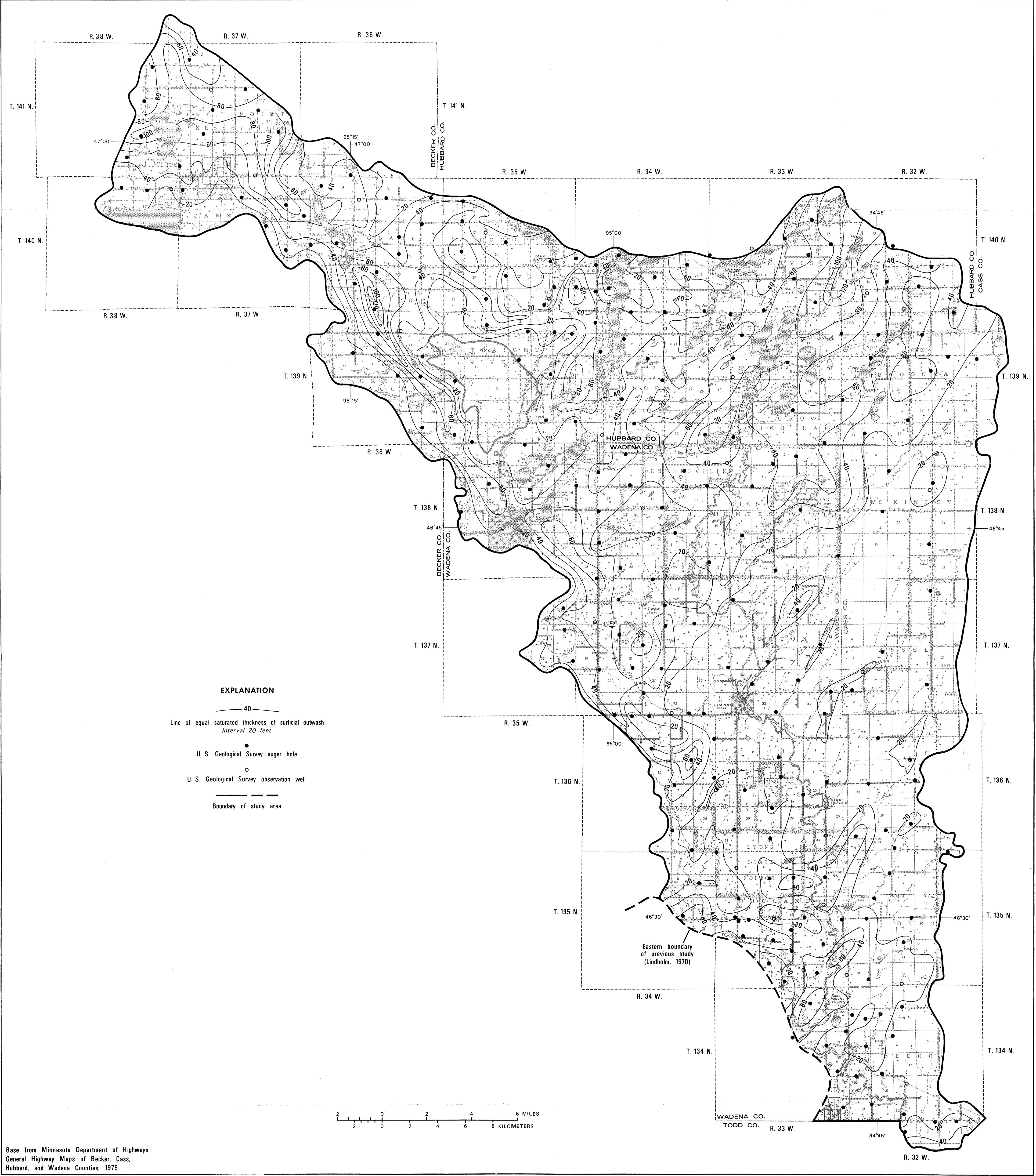
Plate 1.--Saturated thickness of surficial outwash in the Pineland Sands area.
