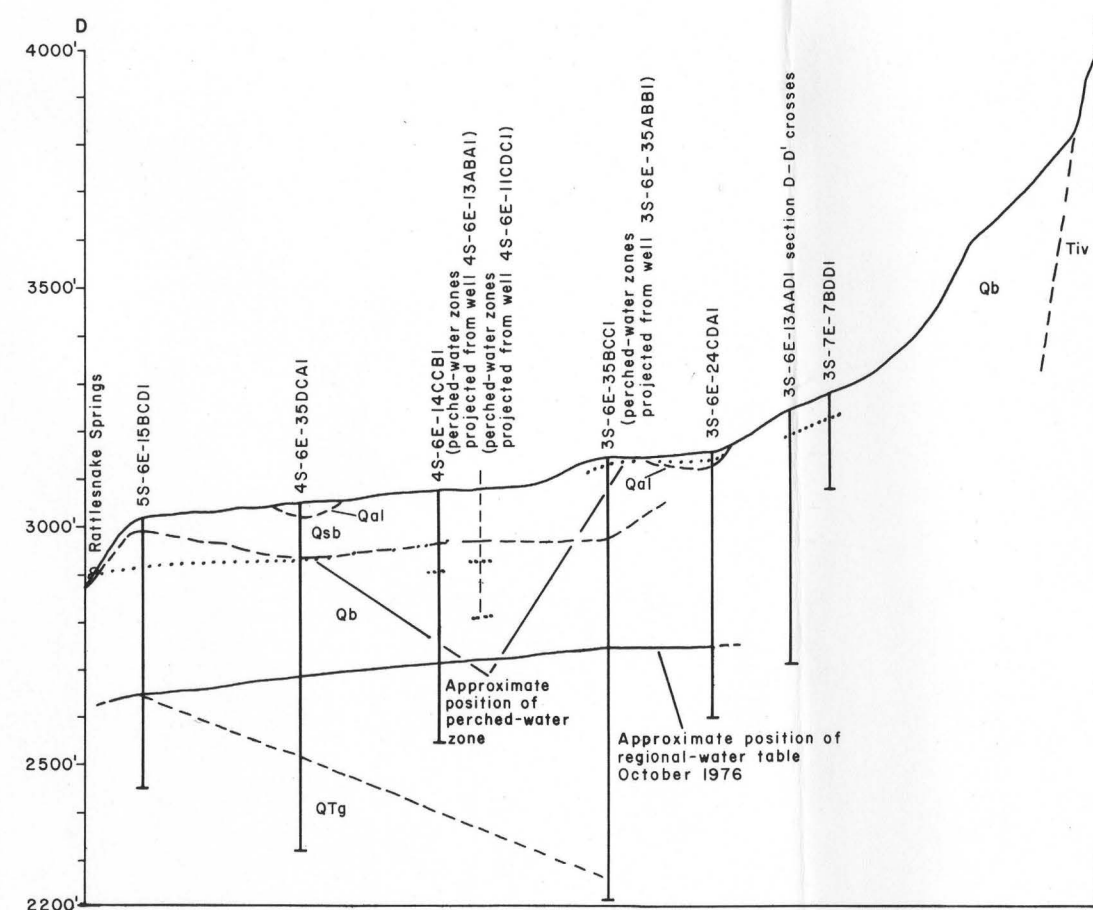
FIGURE 5.--GENERALIZED HYDROGEOLOGIC SECTIONS IN THE MOUNTAIN HOME PLATEAU AREA, IDAHO
