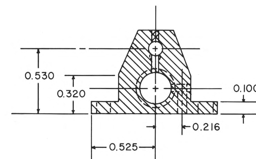
Section C-C
