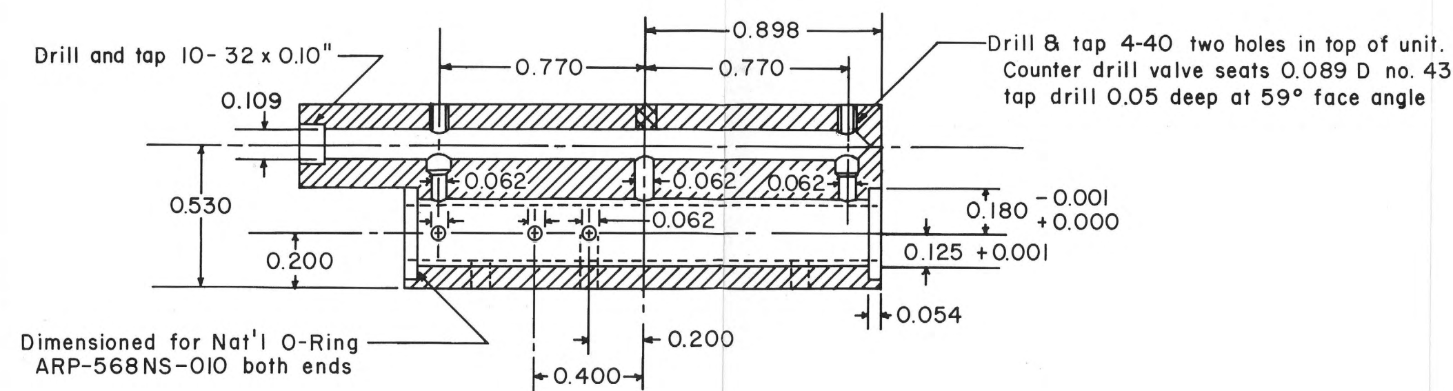
Section B-B
