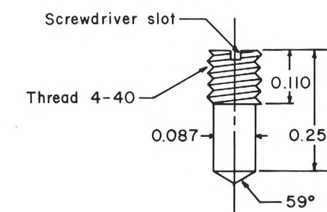
35 Needle valve (2) Scale 1" = 0.2"
