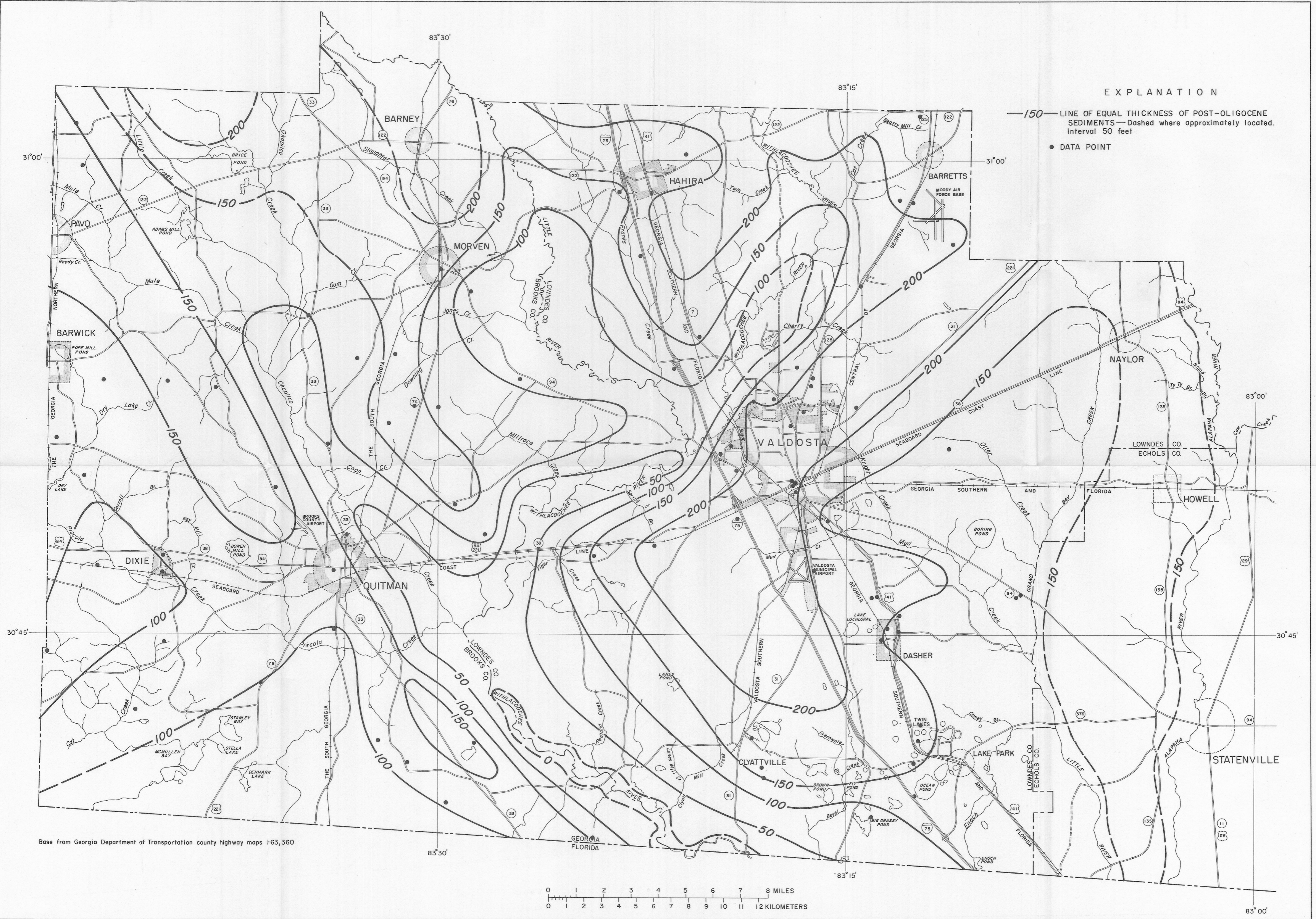
THICKNESS OF POST-OLIGOCENE SEDIMENTS, BROOKS, LOWNDES, AND WESTERN ECHOLS COUNTIES, GEORGIA.
