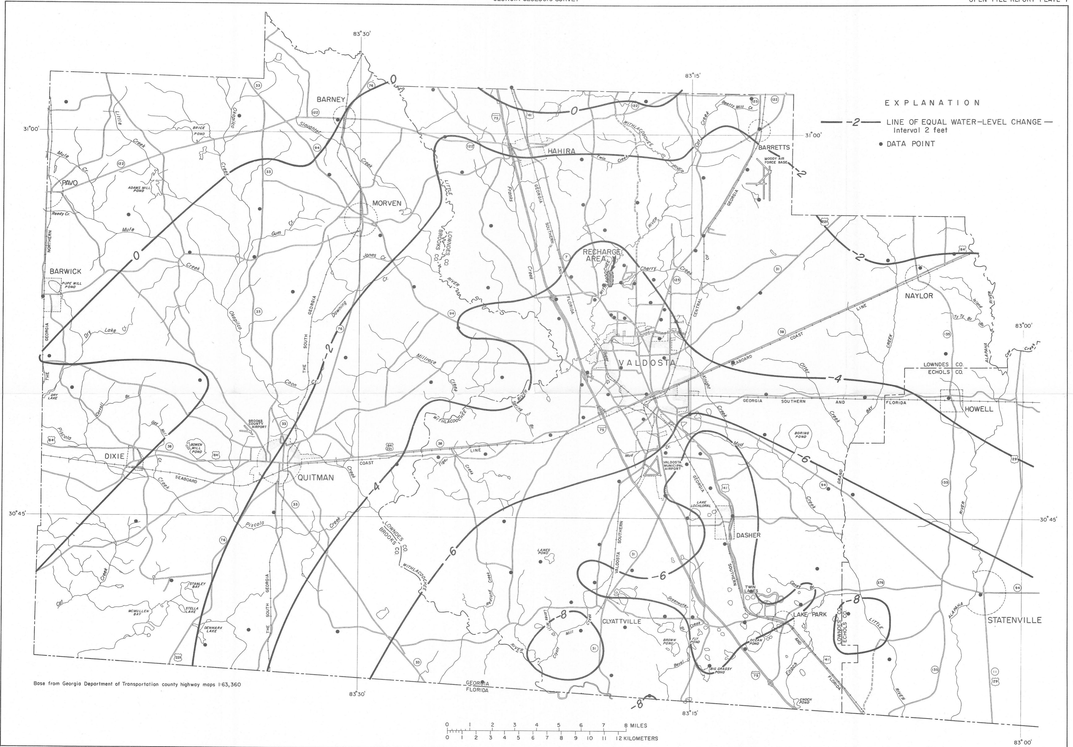
CHANGE IN WATER LEVEL IN WELLS TAPPING THE PRINCIPAL ARTESIAN AQUIFER, BROOKS, LOWNDES, AND WESTERN ECHOLS COUNTIES, GEORGIA, MAY TO NOVEMBER 1975.
