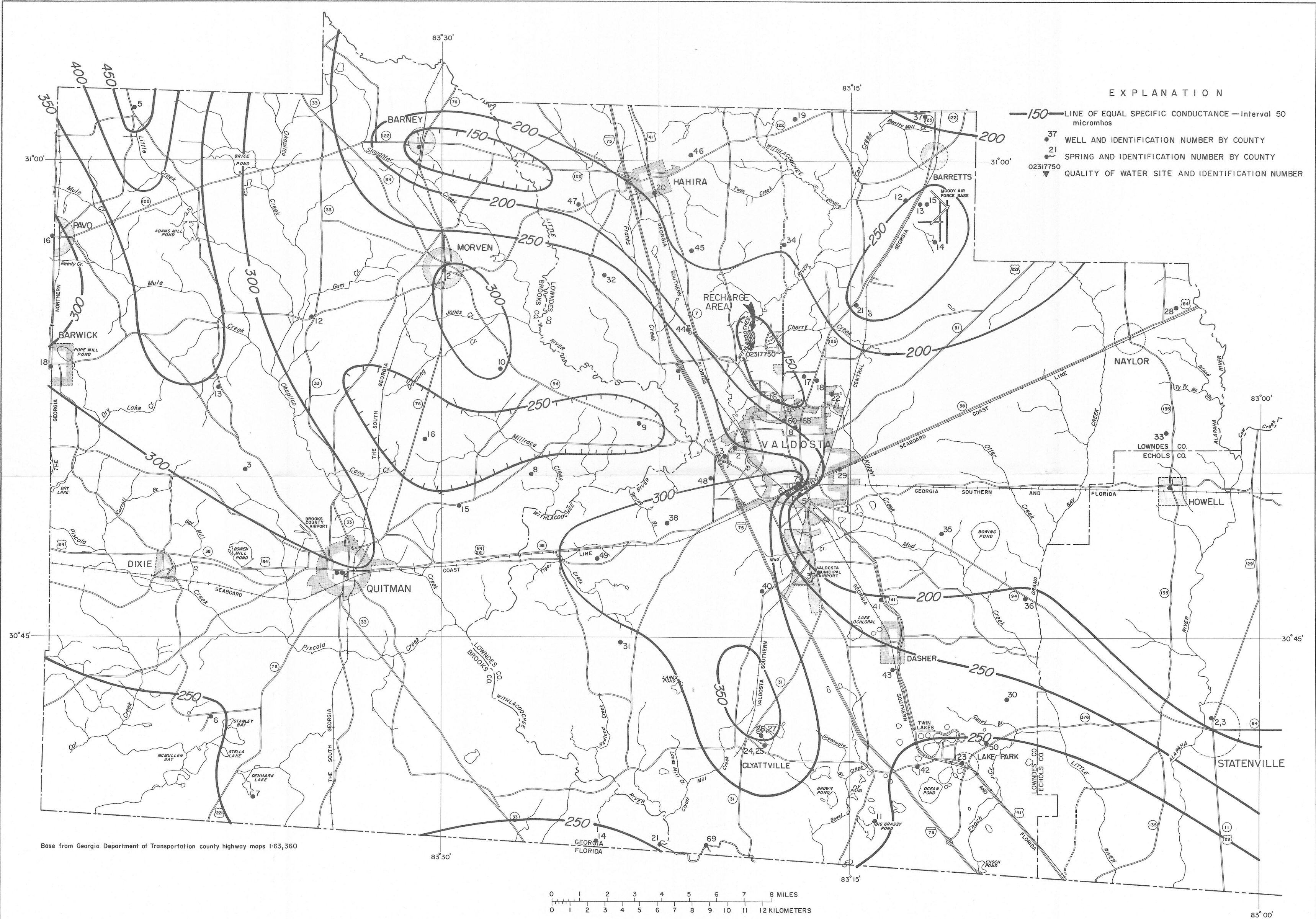
SPECIFIC CONDUCTANCE OF WATER FROM WELLS TAPPING THE PRINCIPAL ARTESIAN AQUIFER, BROOKS, LOWNDES, AND WESTERN ECHOLS COUNTIES, GEORGIA, 1974.
