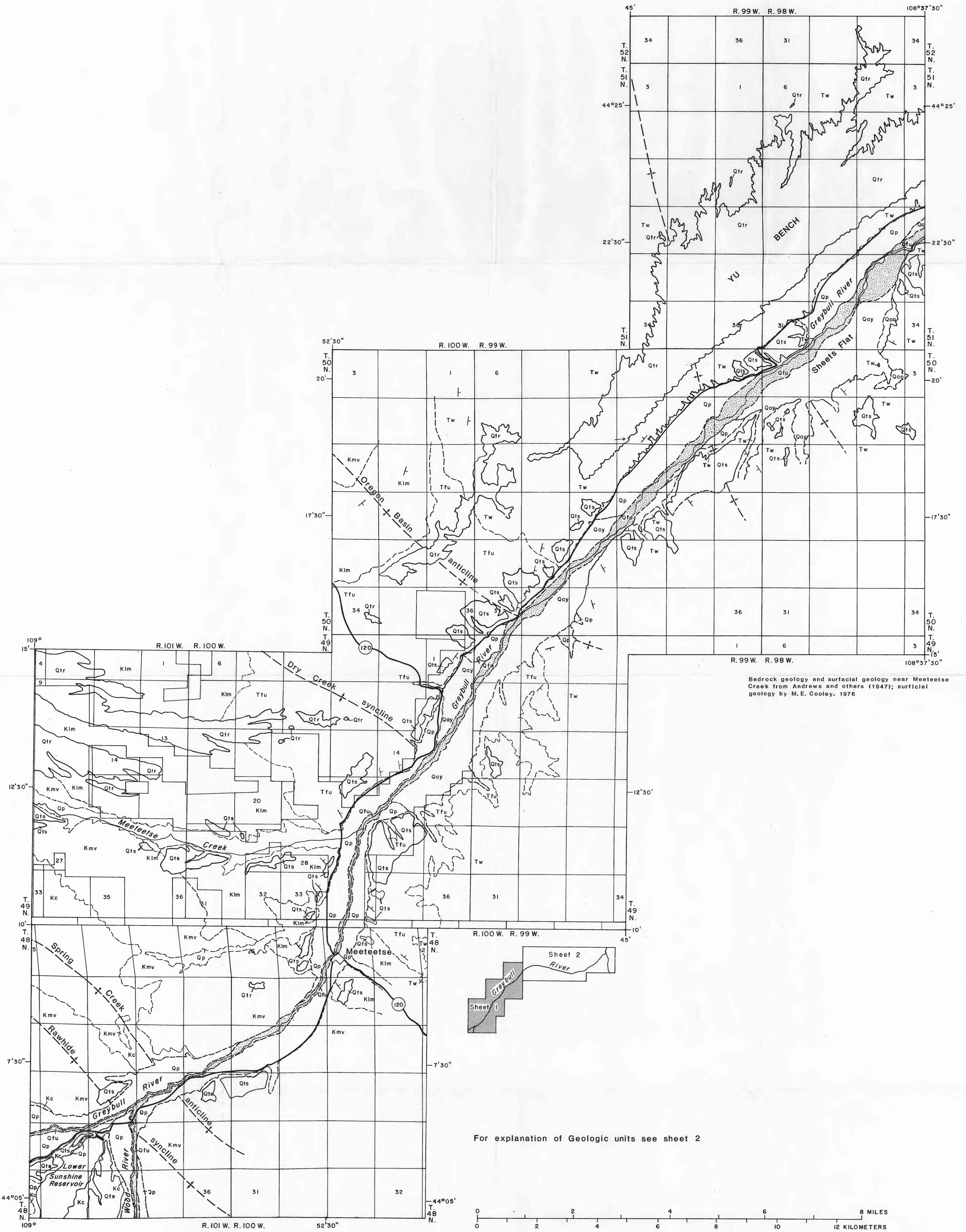
Plate 1. Geologic map showing distribution of the water-yielding and nonwater-yielding alluvial deposits in the Greybull River Valley
