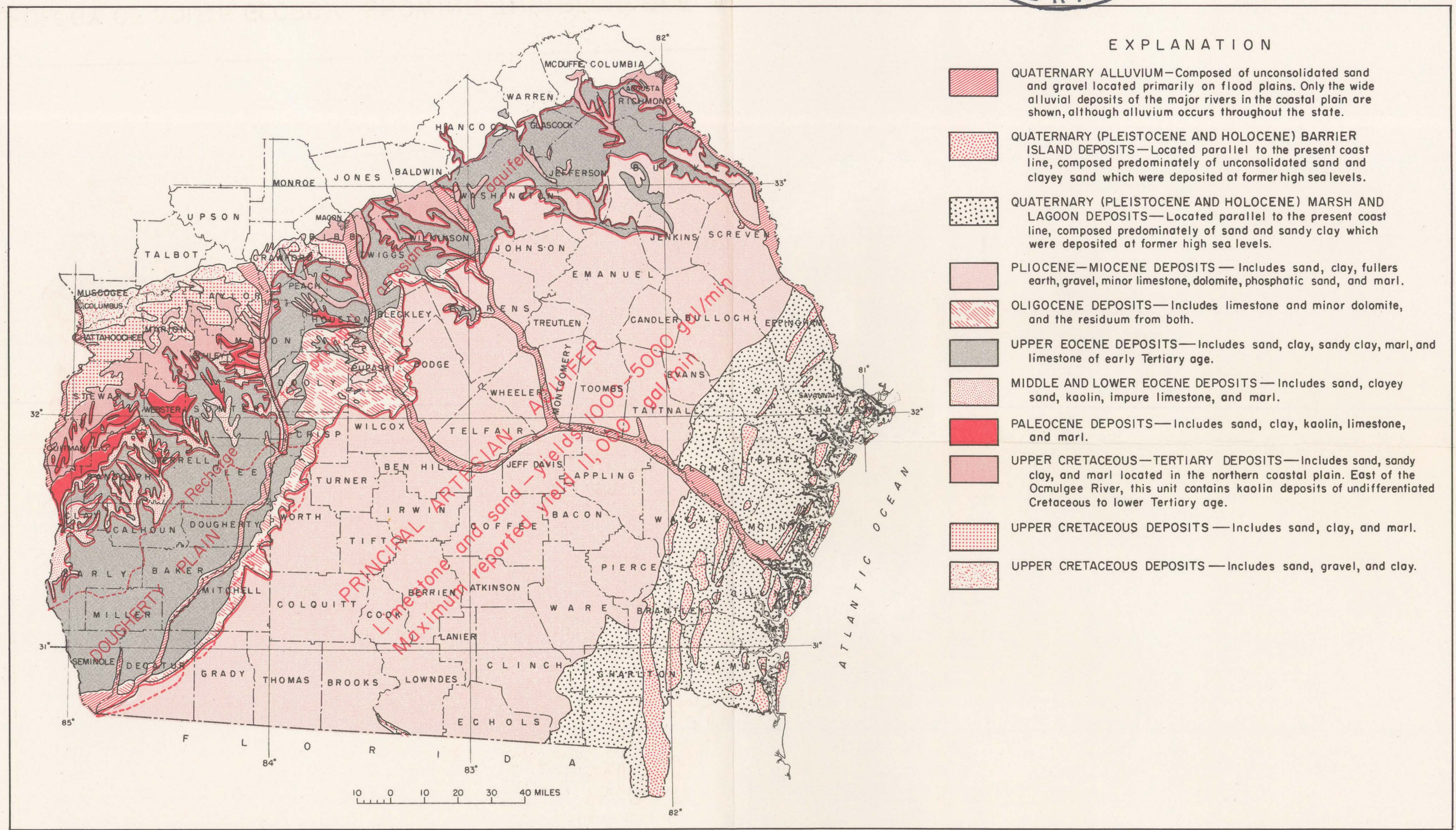
GEOLOGY OF SOUTH GEORGIA SHOWING THE RECHARGE AREA AND AREAL EXTENT OF THE PRINCIPAL ARTESIAN AQUIFER.
