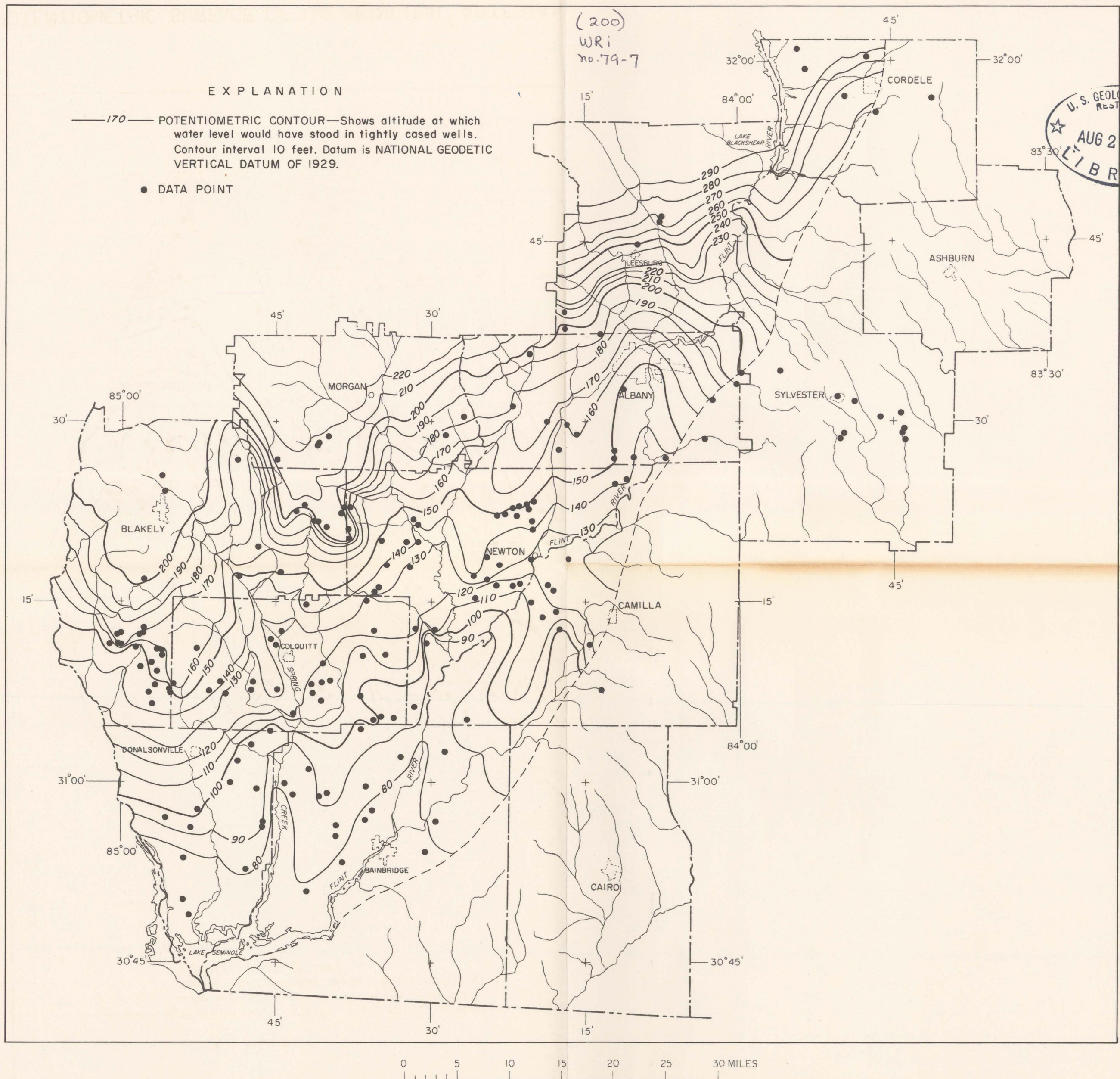
POTENTIOMETRIC SURFACE OF THE PRINCIPAL ARTESIAN AQUIFER, DOUGHERTY PLAIN DISTRICT, NOVEMBER–DECEMBER 1977, SOUTHWEST GEORGIA.
