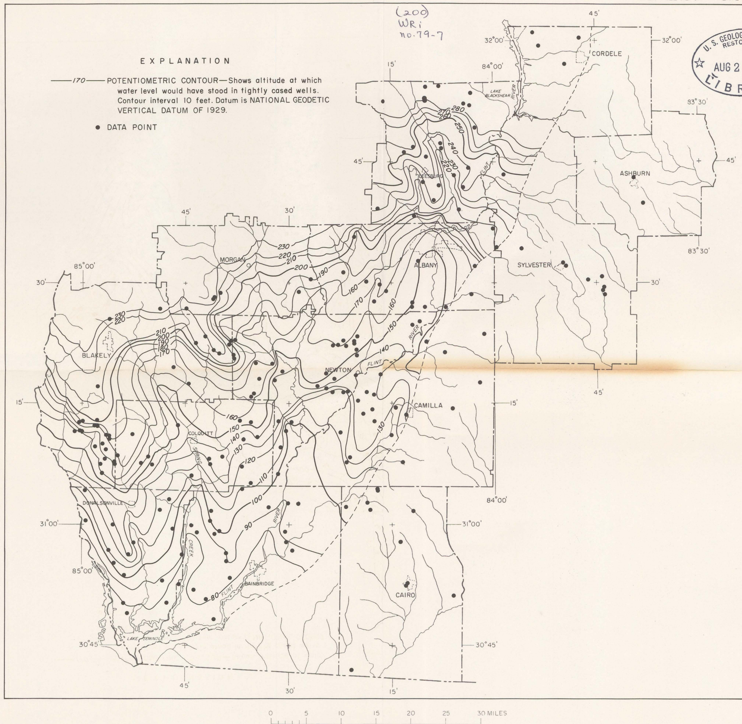
POTENTIOMETRIC SURFACE OF THE PRINCIPAL ARTESIAN AQUIFER, DOUGHERTY PLAIN DISTRICT, MARCH 1978, SOUTHWEST GEORGIA.
