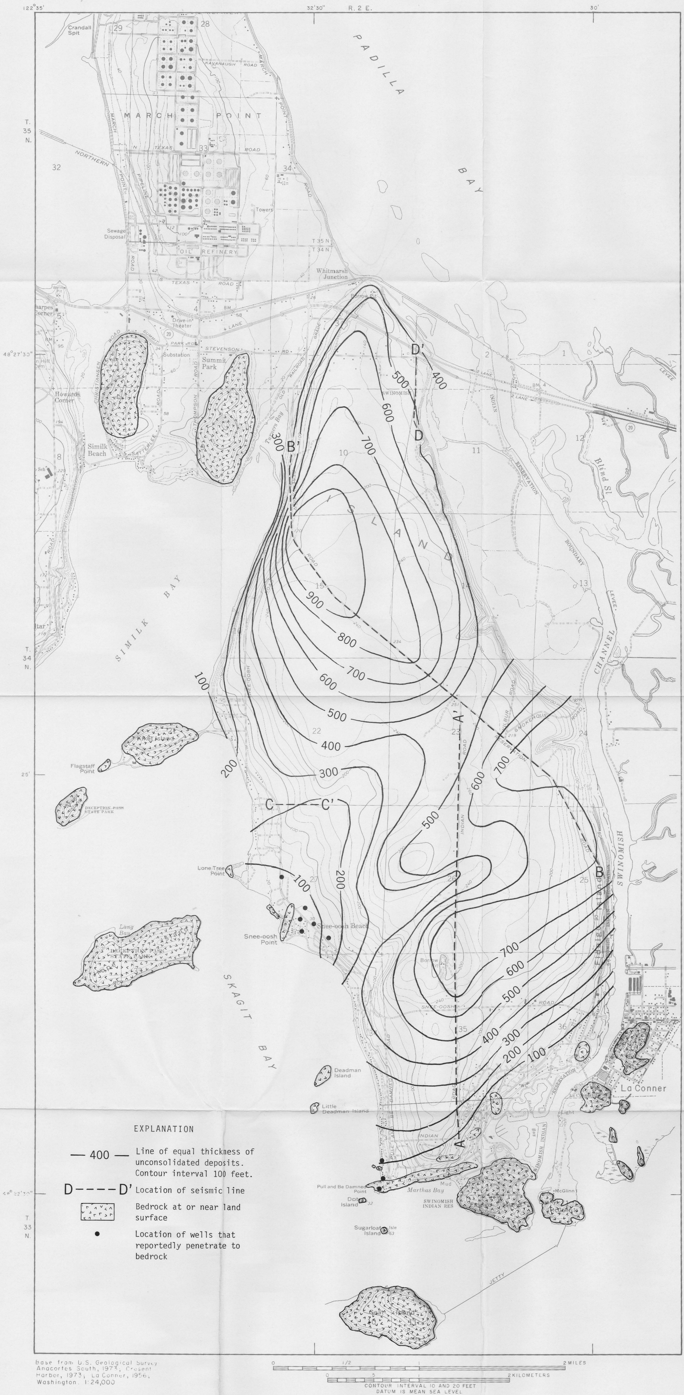
PLATE 3. -- Map of Swinomish Indian Reservation, Washington, showing approximate thickness of unconsolidated deposits and locations of seismic lines.
