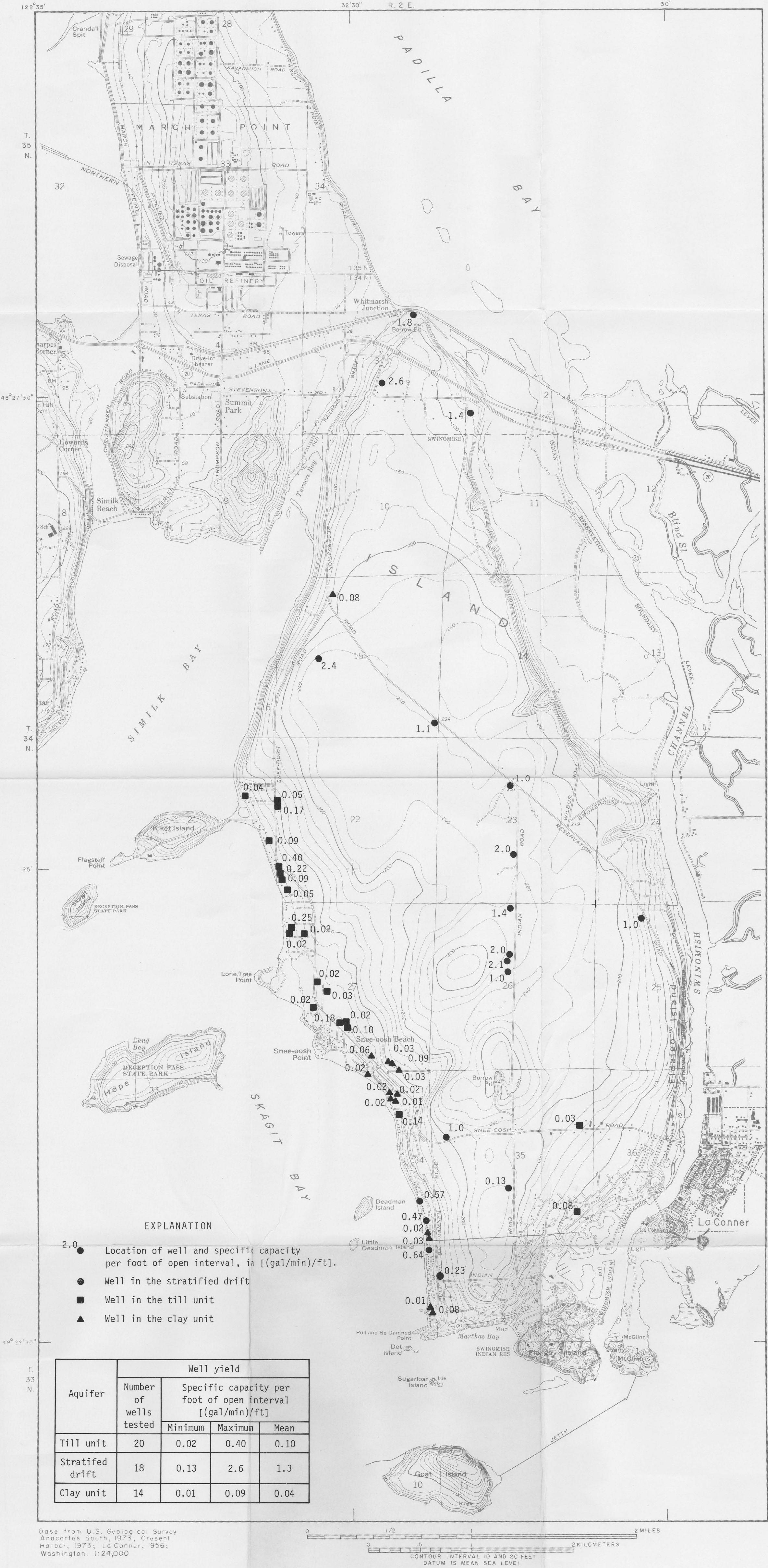
PLATE 5. -- Map of Swinomish Indian Reservation, Washington, showing distribution of specific capacities per foot of open interval in wells tapping the till unit, stratified drift, and clay unit.
