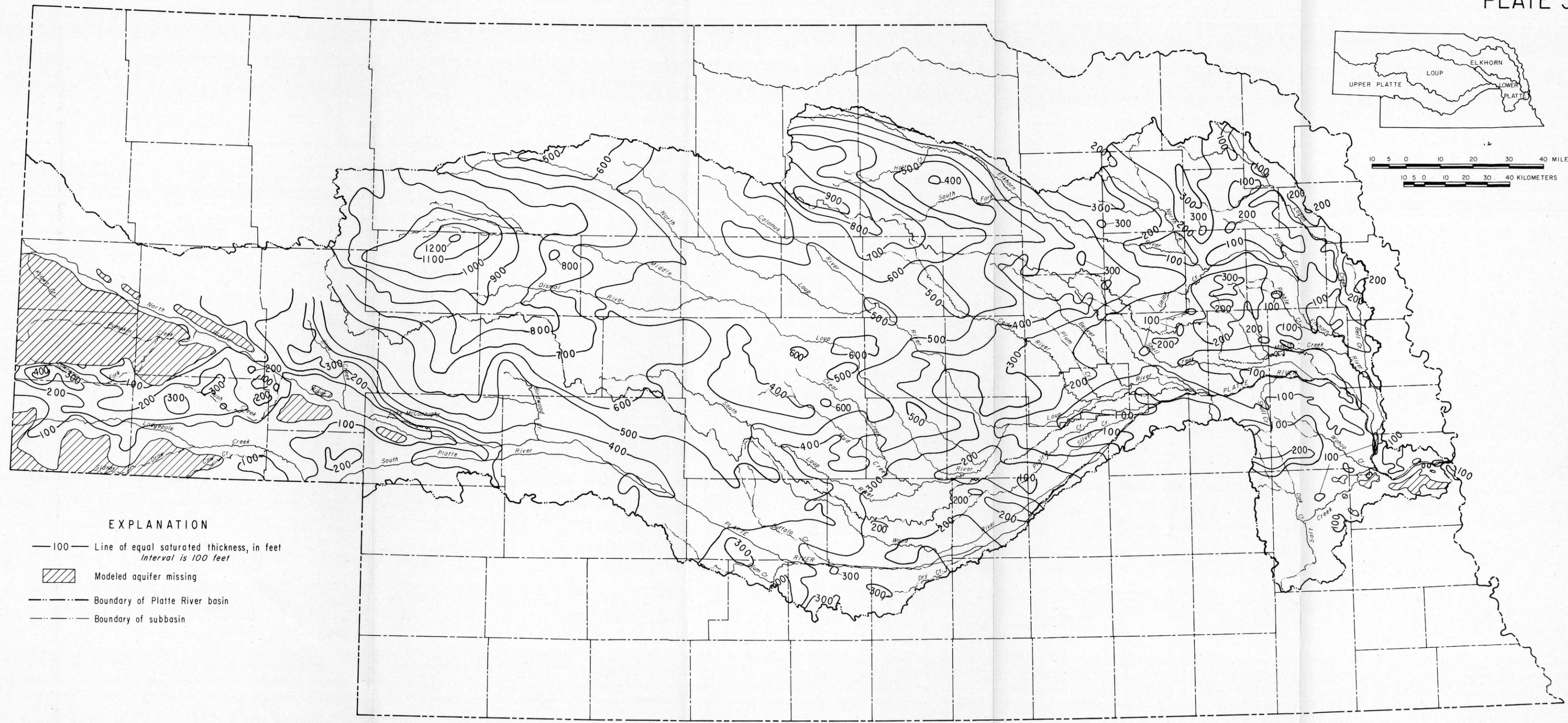
SATURATED THICKNESS OF MODELED AQUIFER
