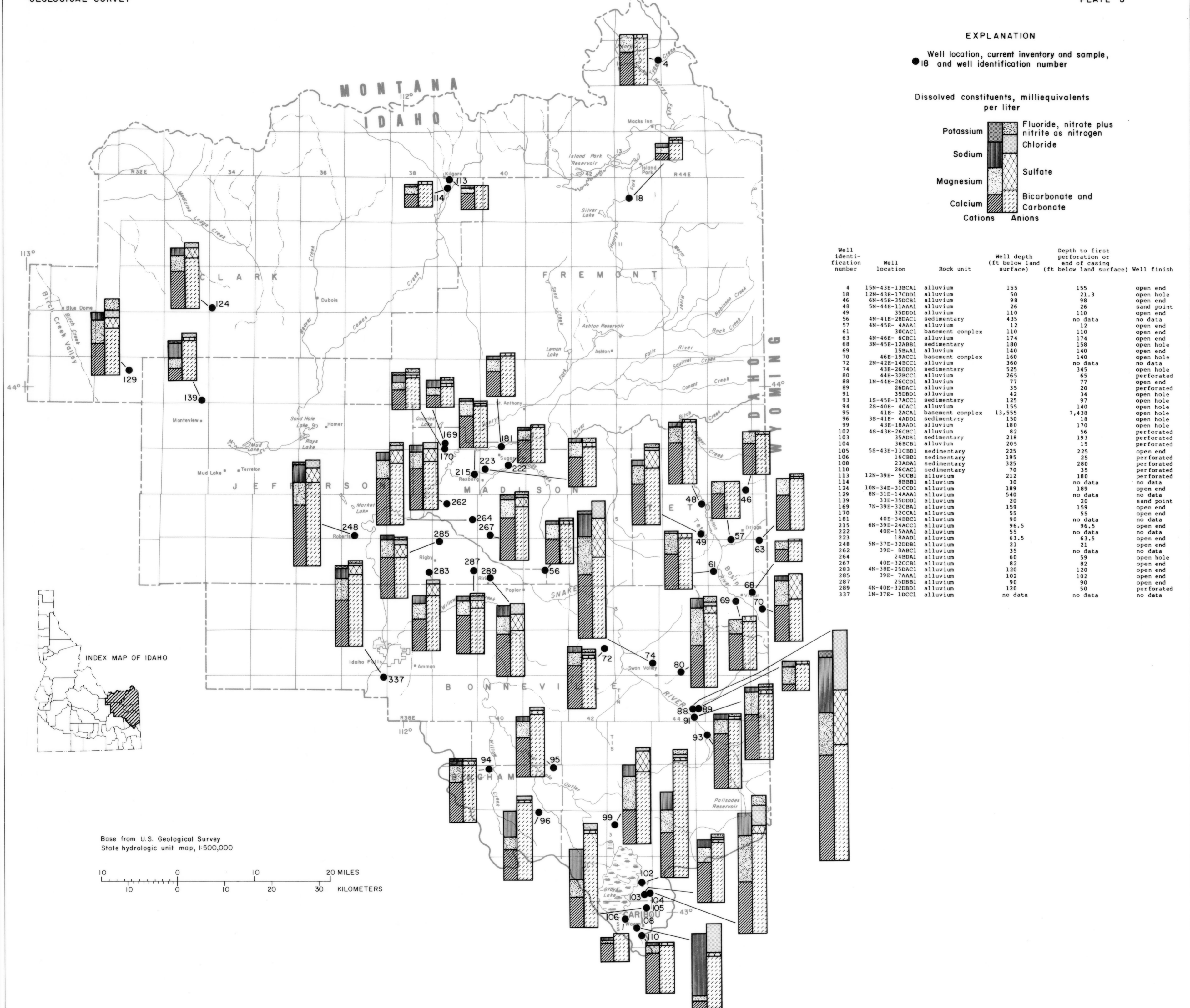
PROPORTIONS OF SELECTED CHEMICAL CONSTITUENTS IN GROUND WATER FROM ALLUVIUM, SEDIMENTARY, AND BASEMENT COMPLEX ROCK UNITS, EASTERN SNAKE RIVER BASIN, IDAHO
