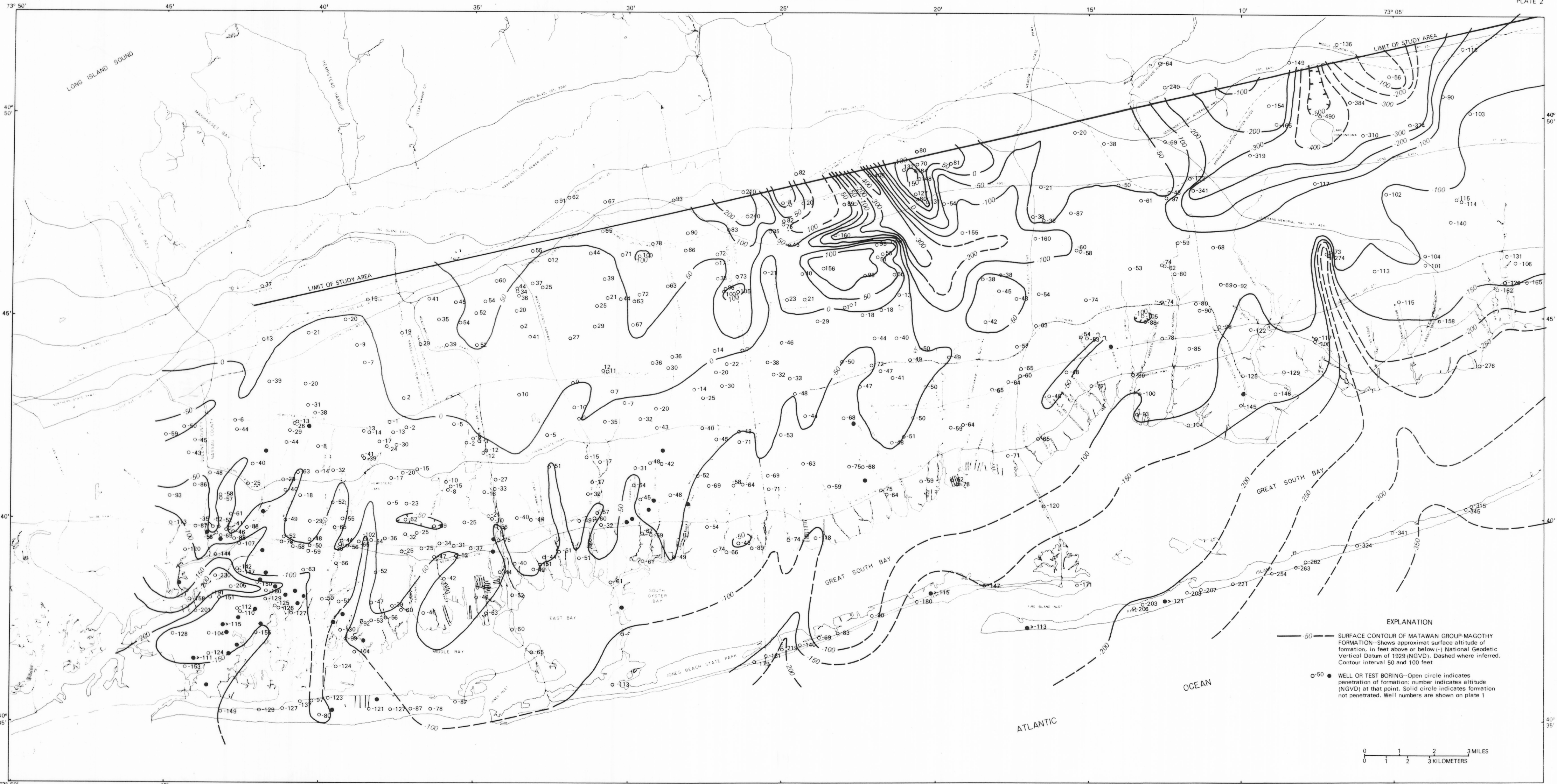
SURFACE ALTITUDE OF MATAWAN GROUP-MAGOTHY FORMATION, UNDIFFERENTIATED IN SOUTHERN NASSAU AND SOUTHWESTERN SUFFOLK COUNTIES, NEW YORK
