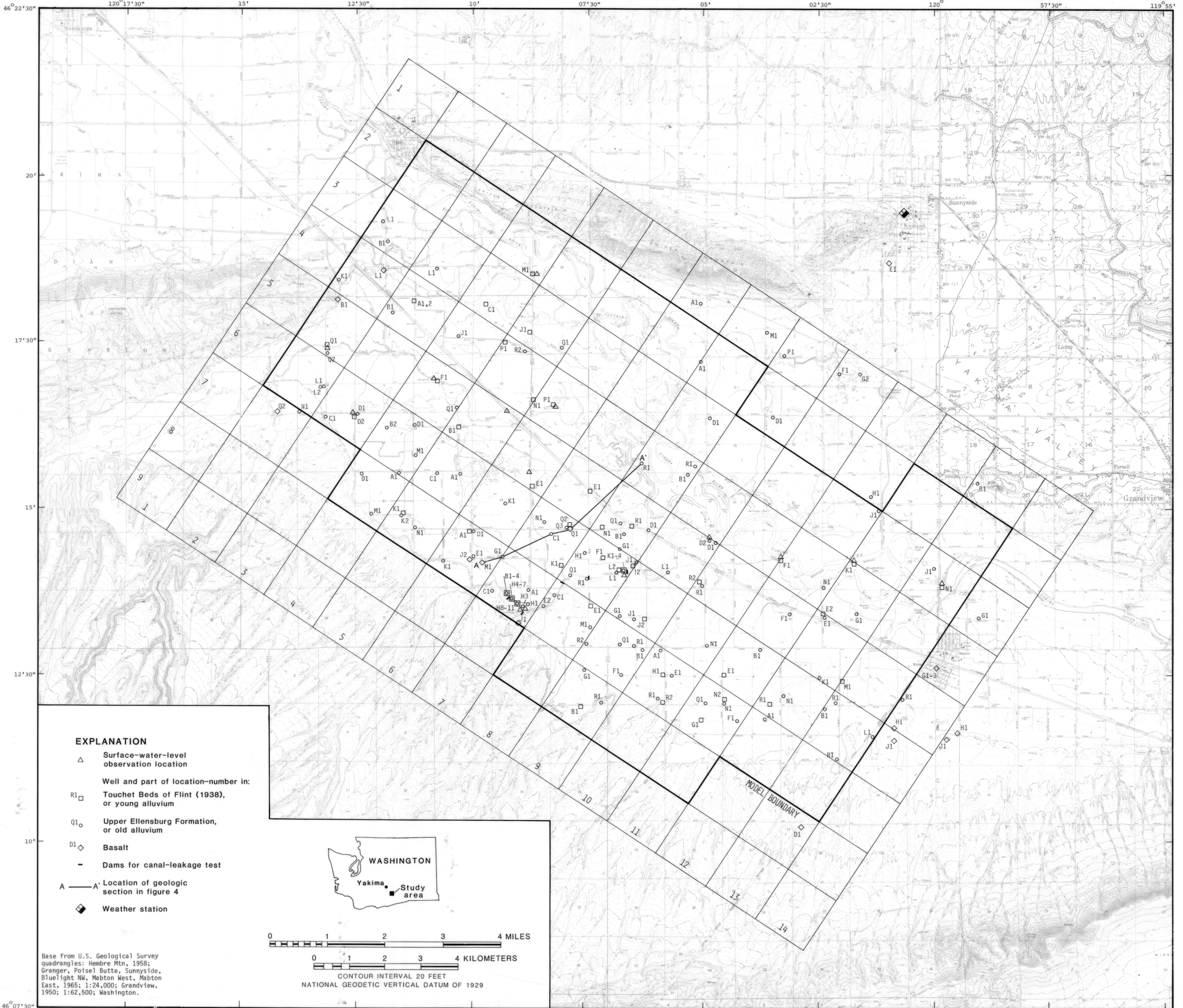
PLATE 1.--Map of Satus Creek basin showing locations of data-collection sites, model grid and boundaries.
